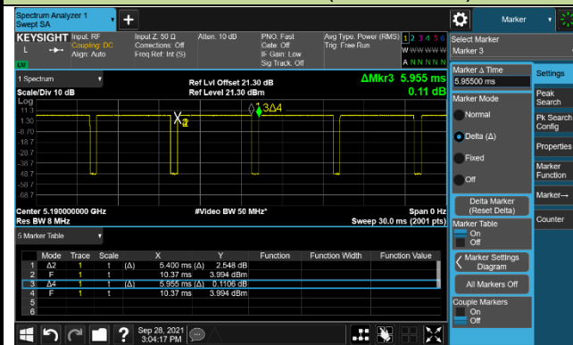
802.11ac-VHT40 (T=5.400ms)
