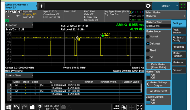
802.11ax-HE80 (T=5.430ms)
