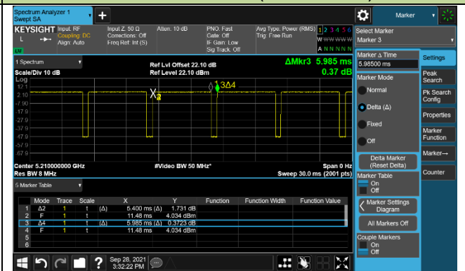
802.11ac-VHT80 (T=5.400ms)
