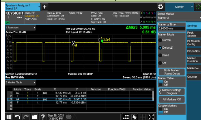
802.11ax-HE160 (T=5.430ms)
