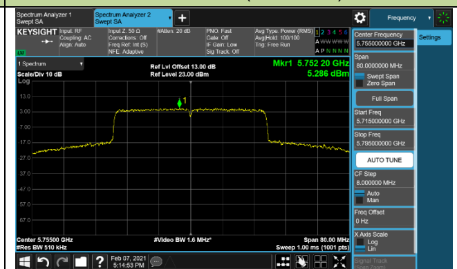
Channel 151 (5755MHz)
