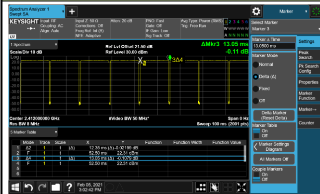
802.11n-HT20 (T = 1.920 ms)
