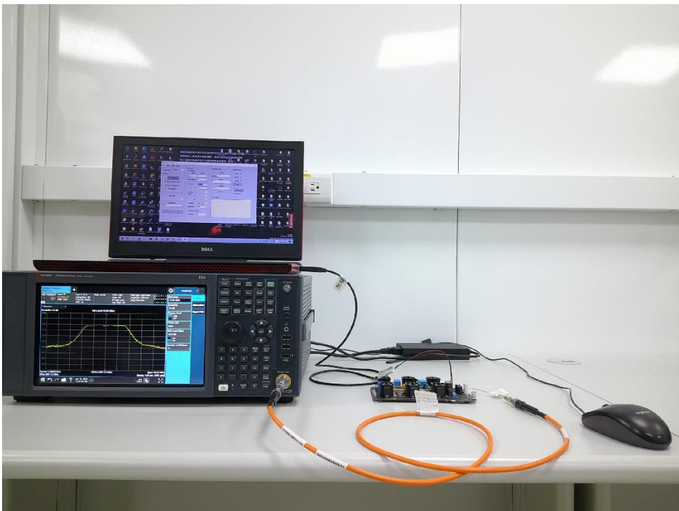
Description: Conducted Emission Test Setup for WiFi
