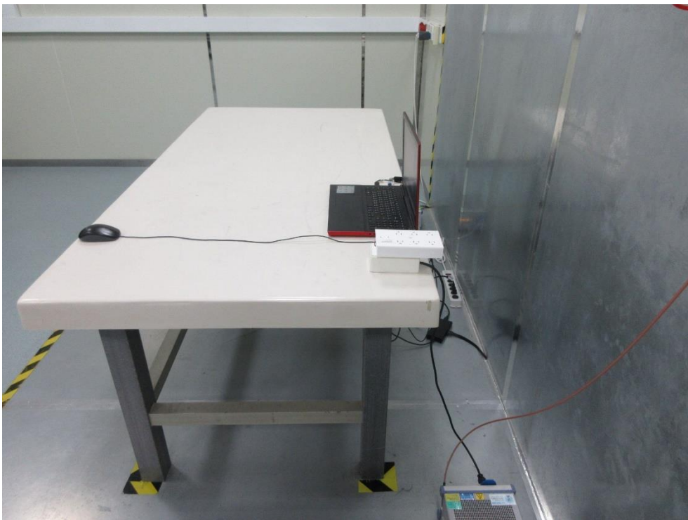
Description: Back View of Conducted Emission Test Setup for WiFi
