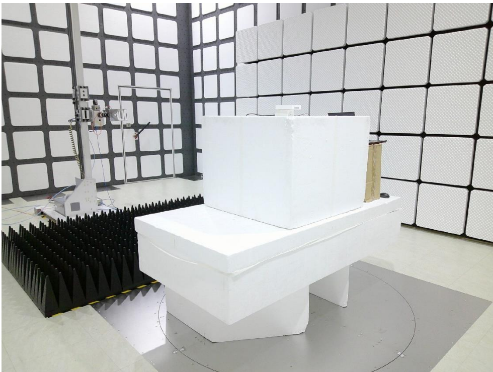
Description: Radiated Emission Test Setup for above 1GHz for BLE
