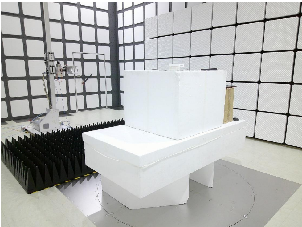
Description: Radiated Emission Test Setup for above 1GHz for WiFi
