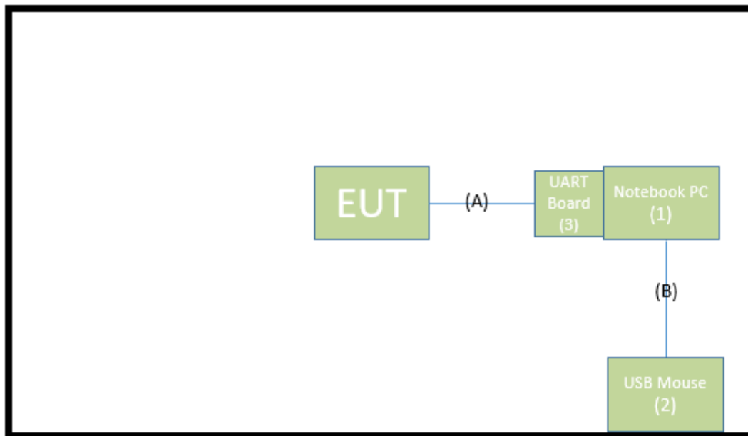
Connection Diagram
