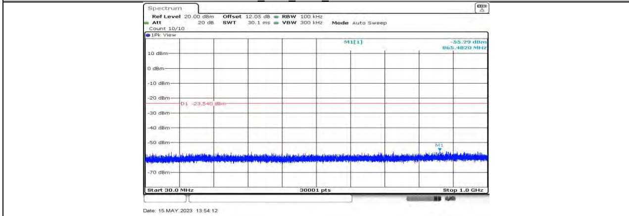
11G_Ant1_2457_30~1000
