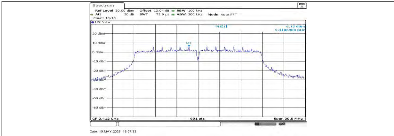
11N20SISO Ant1 2412 0~Reference
