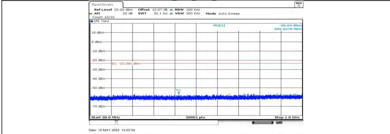
11N20SISO Ant1 2437 30~1000
