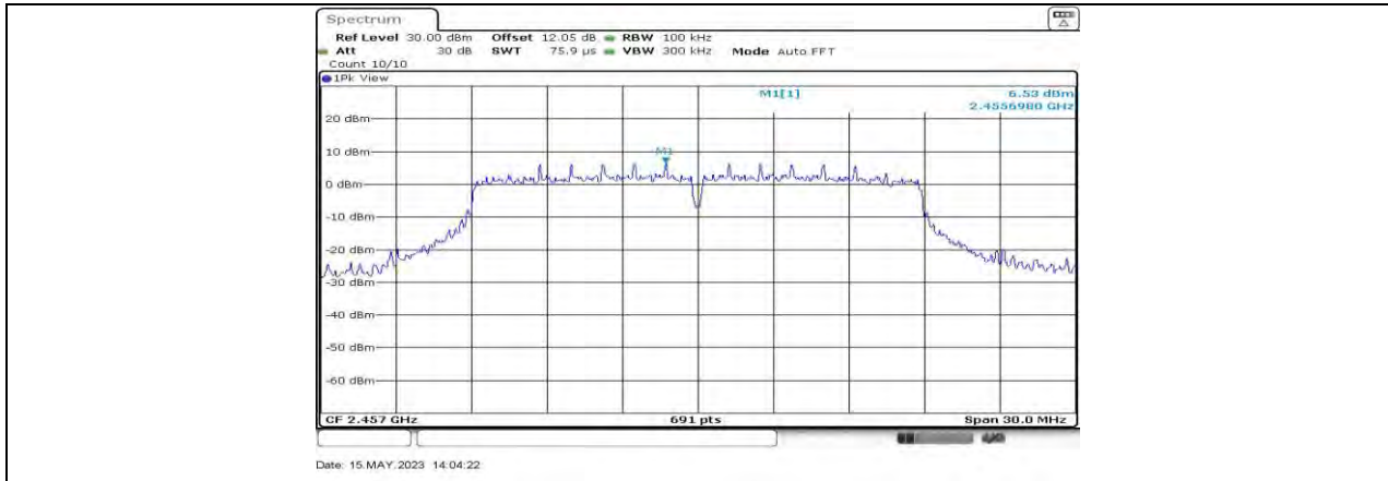
11N20SISO Ant1 2457 0~Reference
