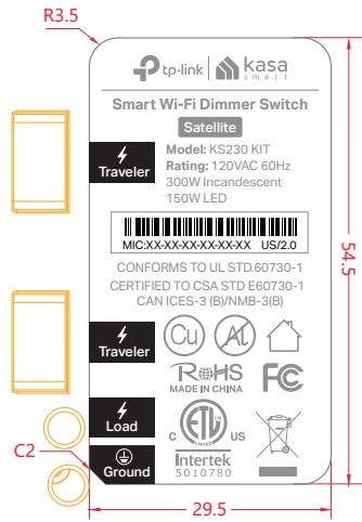
标贴尺寸: 29.5*54.5mm ±0.2, C2, R3.5
