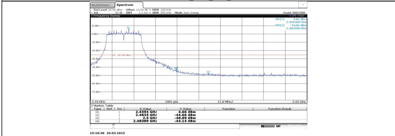
11N20SISO_Ant1_High_2457
