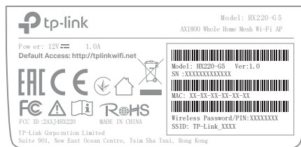
56.7*27.7mm ±0.2
