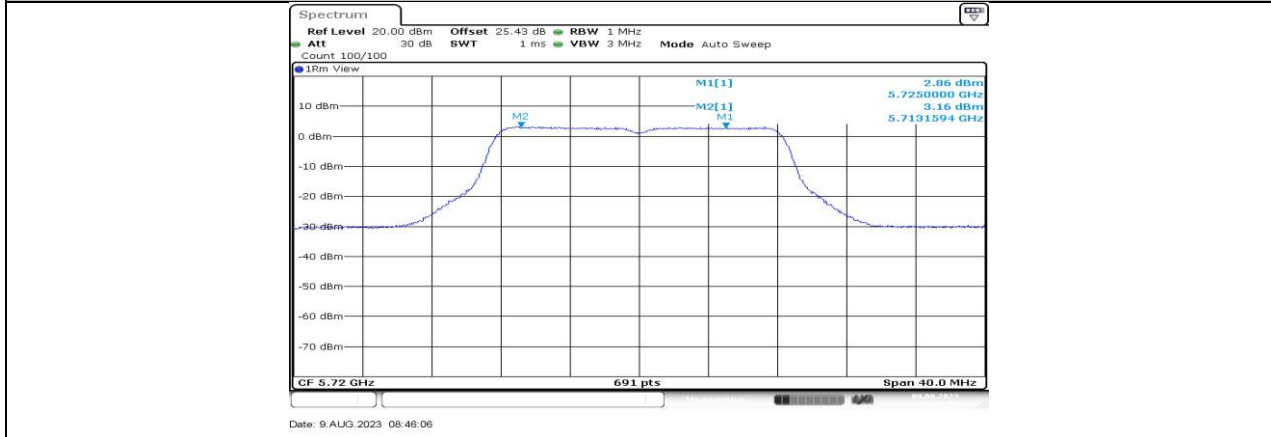
11A-CDD_Ant4_5720_UNII-2C
