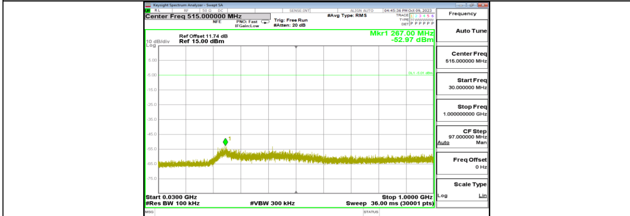
BLE_1M_Ant5_2440_30~1000
