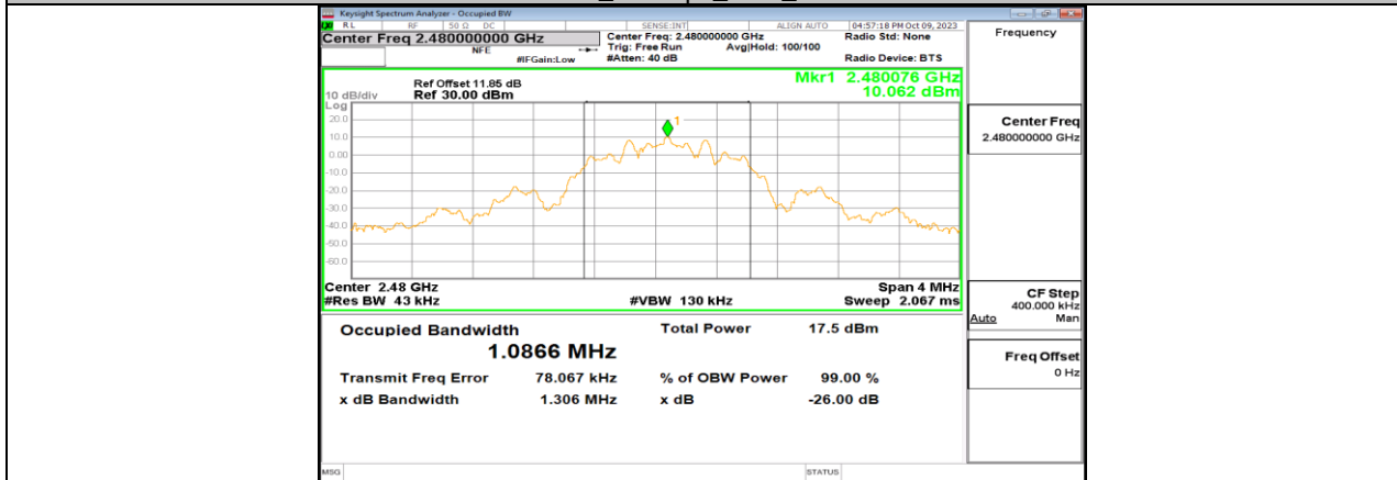
BLE_125kbps_Ant5_2480
