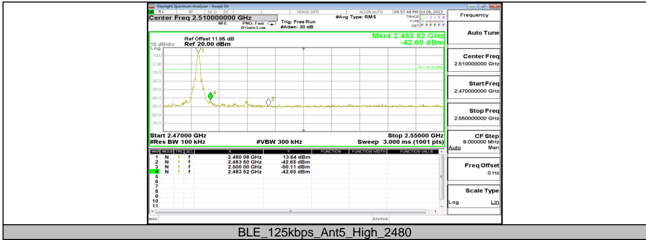
BLE_125kbps_Ant5_High_2480
