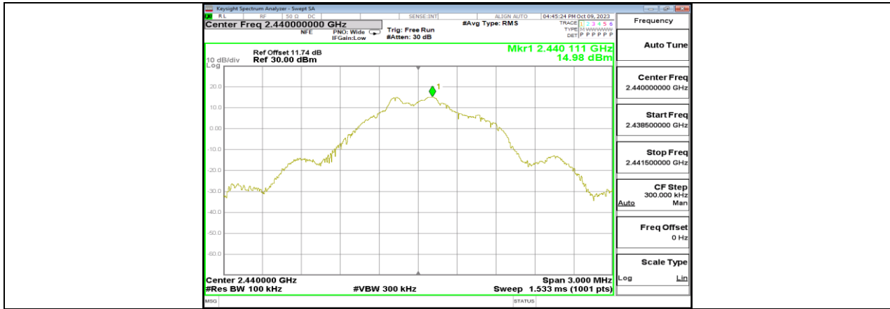
BLE_1M_Ant5_2440_0~Reference
