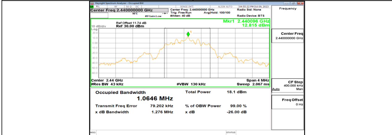
BLE_125kbps_Ant5_2440
