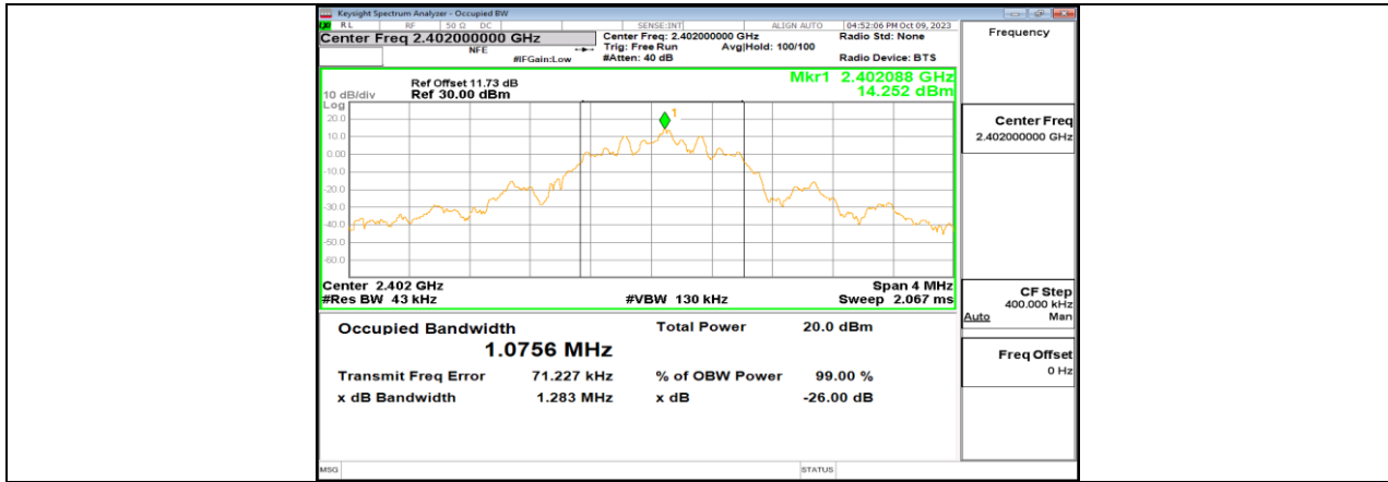
BLE_125kbps_Ant5_2402
