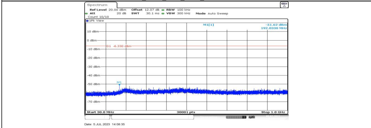
BLE_125K_Ant3_2440_30~1000
