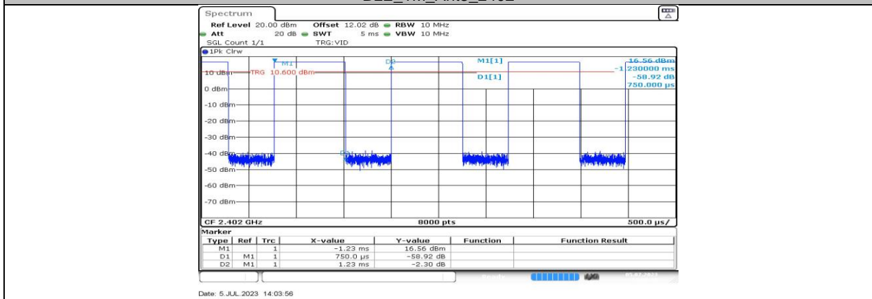
BLE_125K_Ant3_2402
