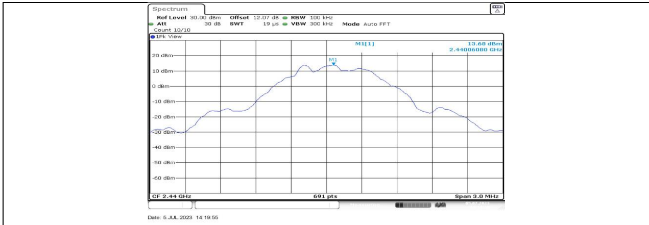
BLE_500K_Ant3_2440_0-Reference
