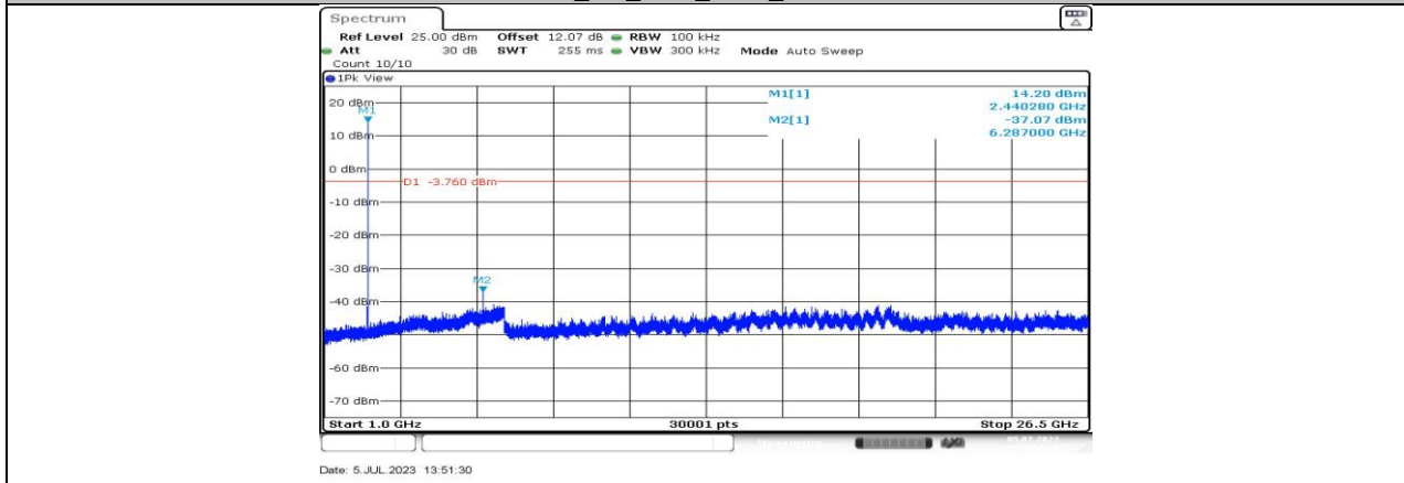
BLE_1M_Ant3_2440_1000~26500
