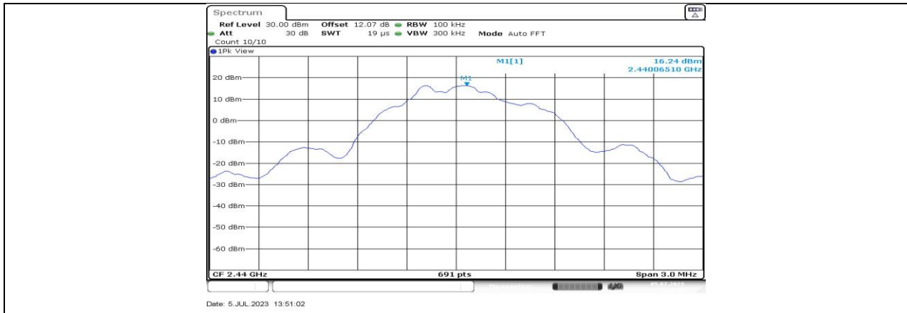
BLE_1M_Ant3_2440_0~Reference
