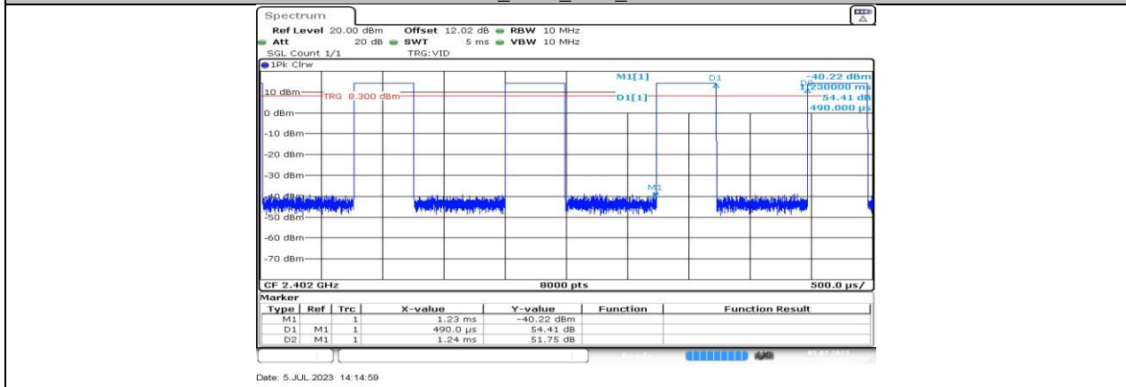
BLE_500K_Ant3_2402
