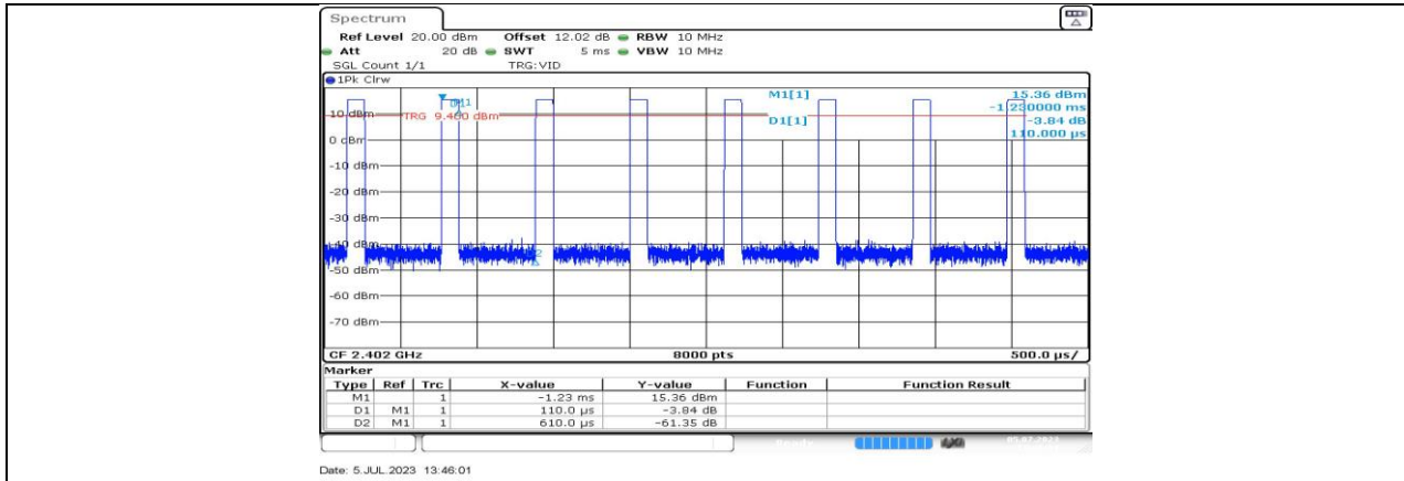
BLE_1M_Ant3_2402
