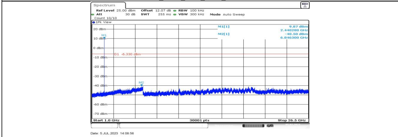
BLE_125K_Ant3_2440_1000~26500
