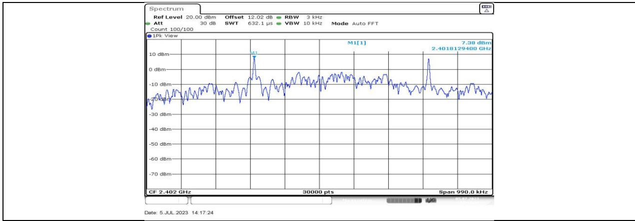
BLE_500K_Ant3_2402
