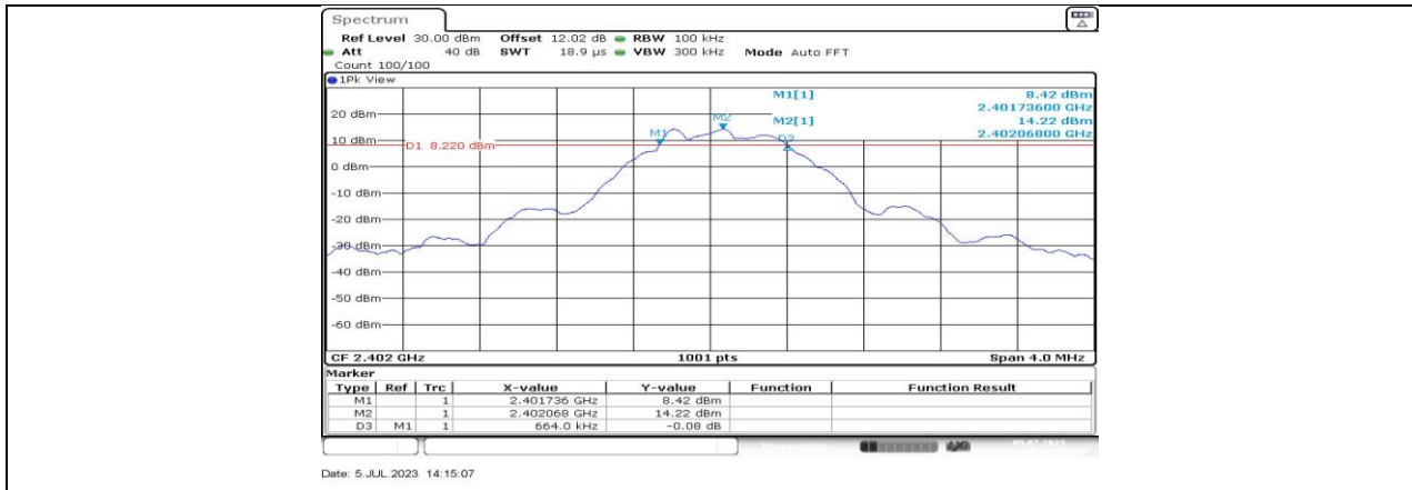
BLE_500K_Ant3_2402
