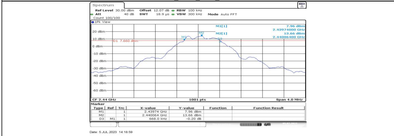
BLE_500K_Ant3_2440
