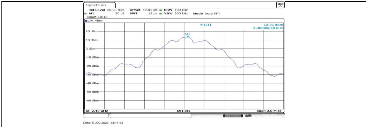
BLE_125K_Ant3_2480_0-Reference
