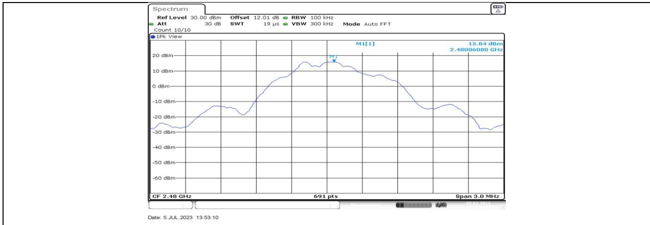
BLE_1M_Ant3_2480_0~Reference
