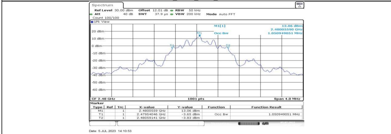
BLE_125K_Ant3_2480
