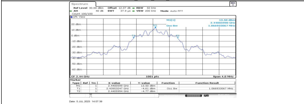
BLE_125K_Ant3_2440
