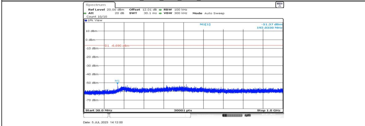
BLE_125K_Ant3_2480_30~1000
