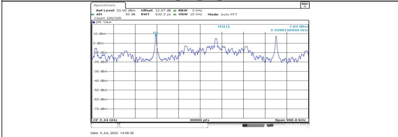
BLE_125K_Ant3_2440
