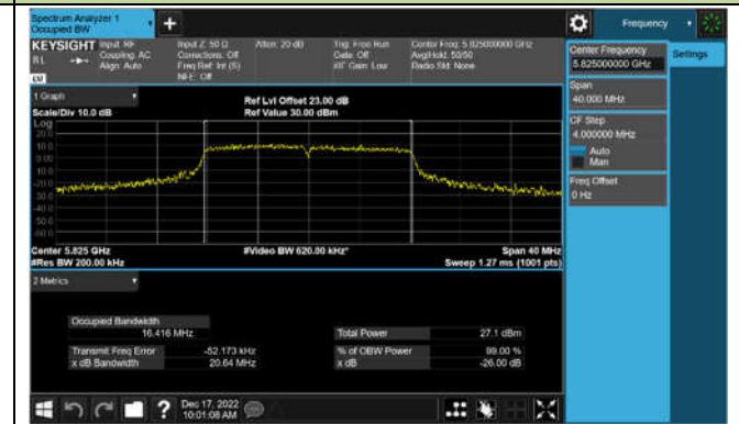
Channel 165 (5825MHz)
