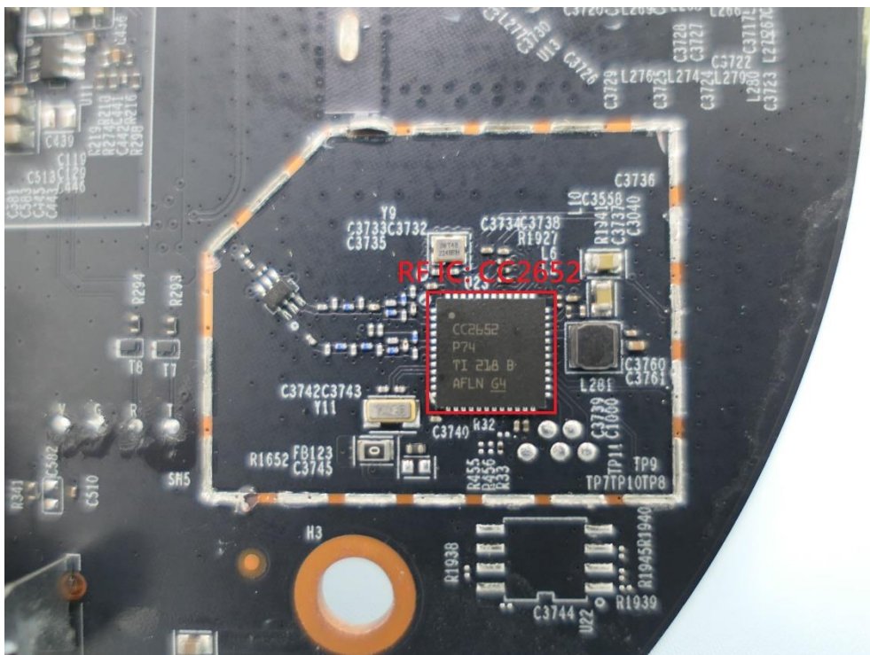
(10) EUT Photo (Mode name: EAP650)
