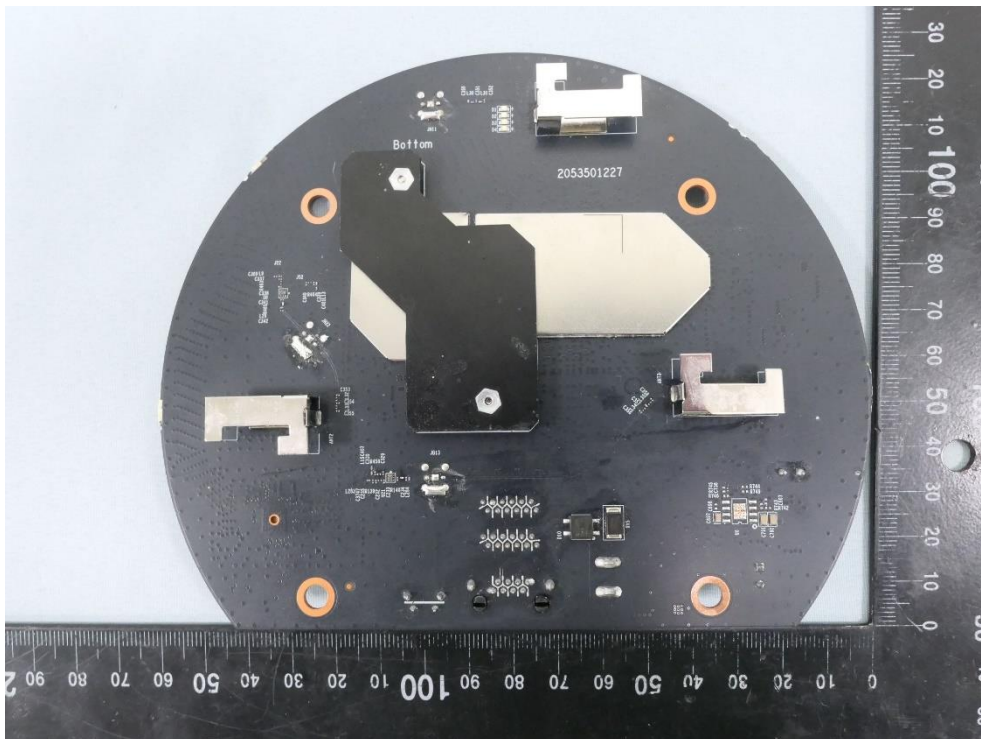
(22) EUT Photo (Mode name: EAP653)
