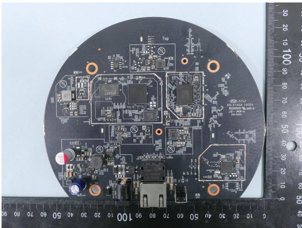
(18) EUT Photo (Mode name: EAP653)
