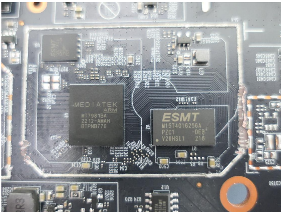
(8) EUT Photo (Mode name: EAP650)
