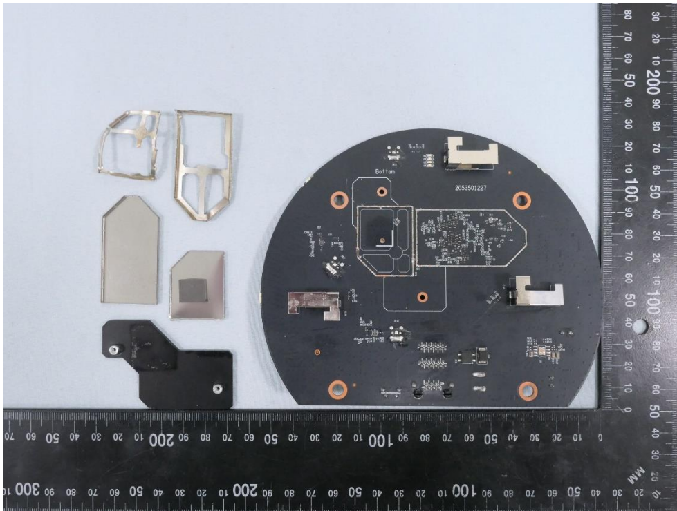
(24) EUT Photo (Mode name: EAP653)
