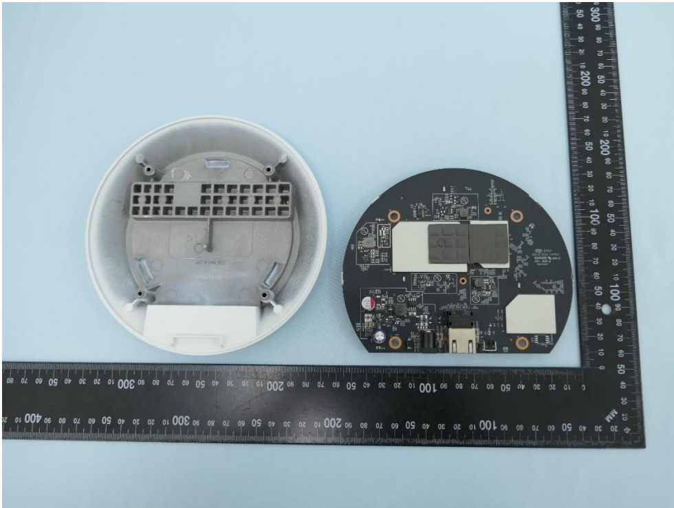
(4) EUT Photo (Mode name: EAP650)
