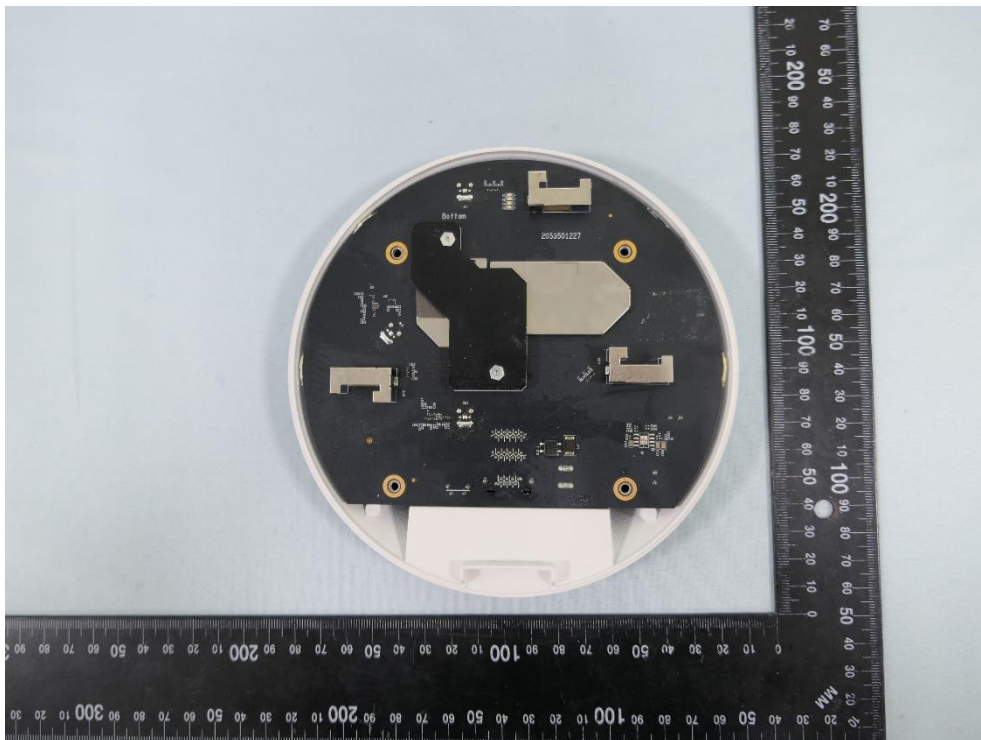
(2) EUT Photo (Mode name: EAP650)
