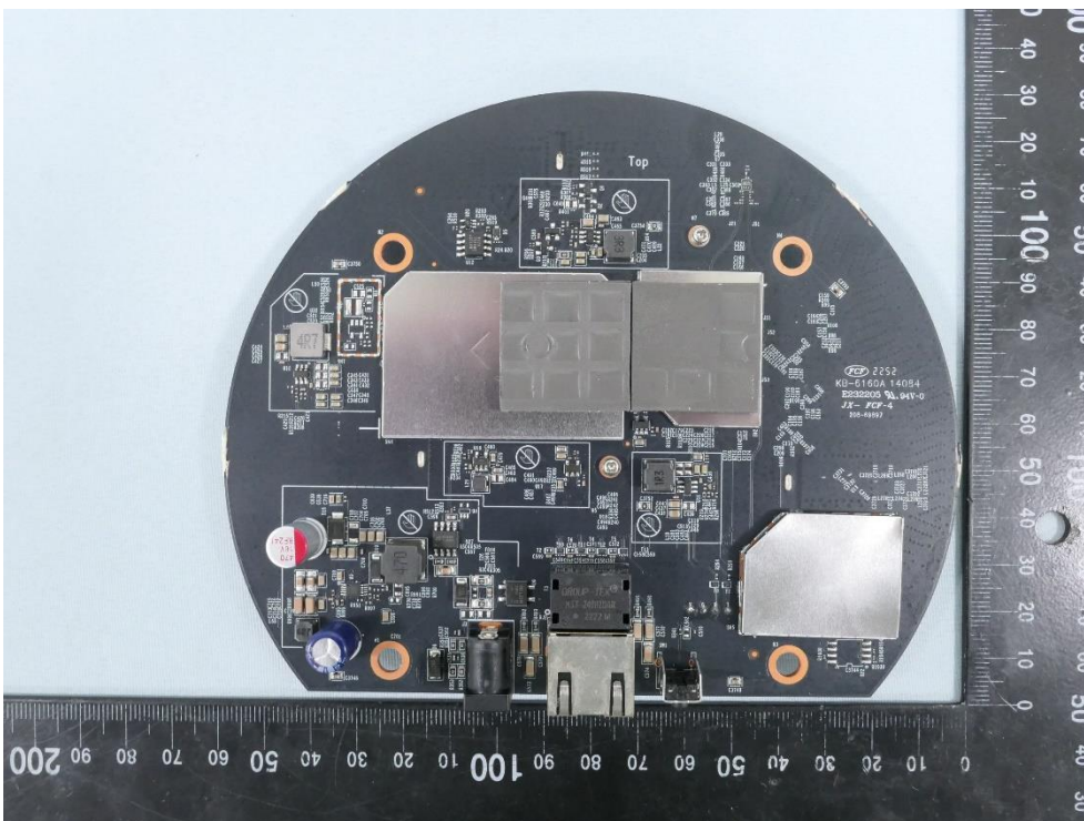
(16) EUT Photo (Mode name: EAP653)
