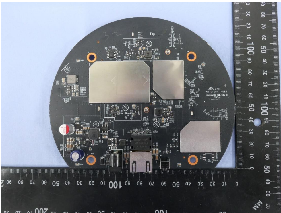
(30) EUT Photo (Mode name: Festa F65)
