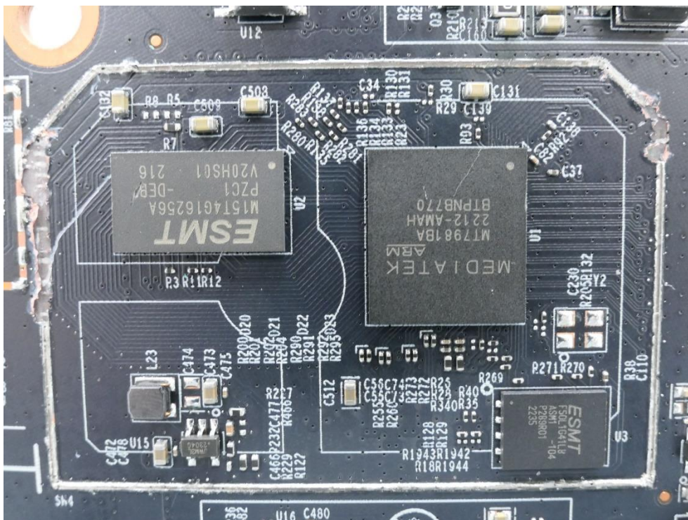
(20) EUT Photo (Mode name: EAP653)
