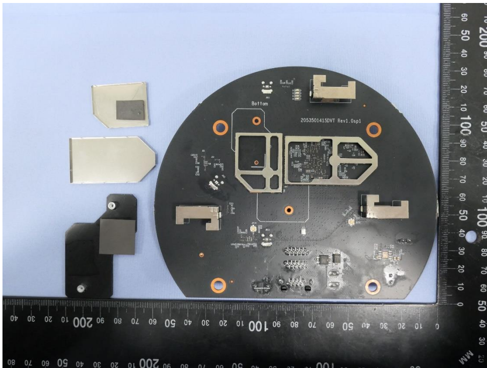
(28) EUT Photo (Mode name: Festa F65)
