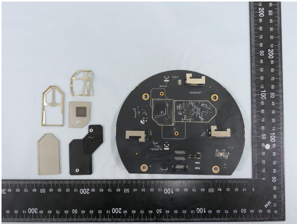
(12) EUT Photo (Mode name: EAP650)
