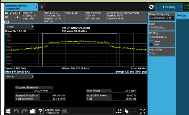
Channel 144 (5785MHz)
