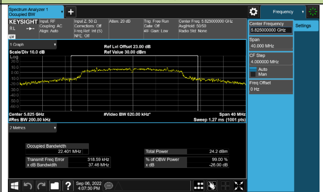
Channel 144 (5825MHz)
