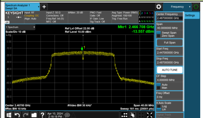
Channel 12 (2467MHz)
