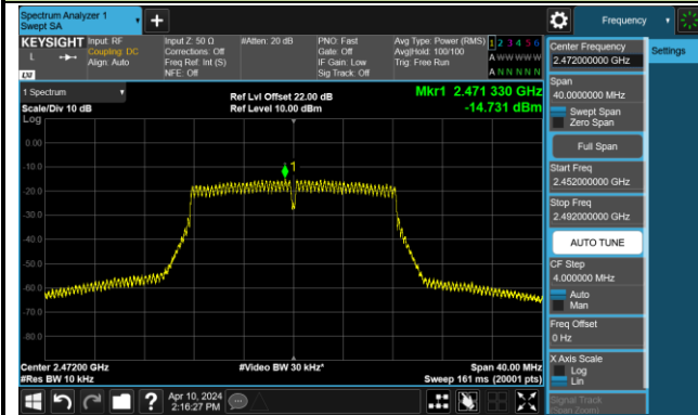
Channel 13 (2472MHz)
