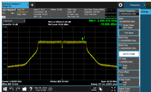
Channel 11 (2462MHz)
