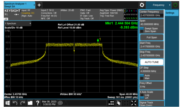
Channel 06 (2437MHz)
