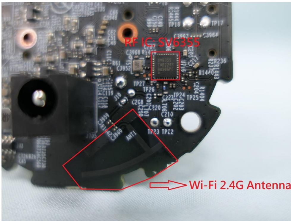
(11) EUT Photo
