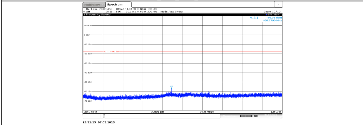
11G-CDD_Ant7_2437_30~1000
