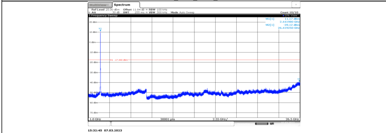
11G-CDD_Ant7_2437_1000~26500
