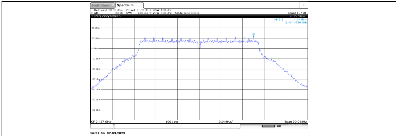
11G-CDD_Ant7_2457_0~Reference
