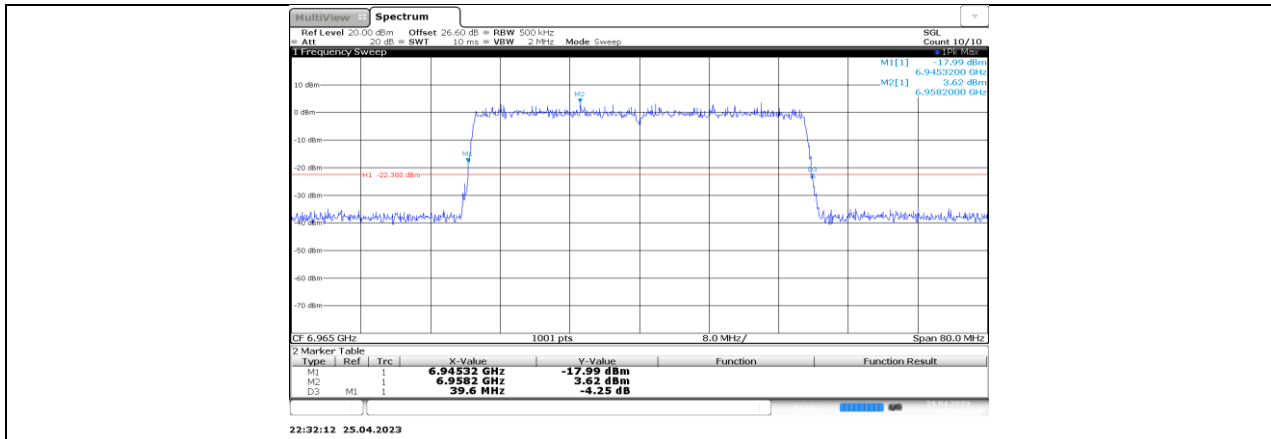
11AX40-CDD_Ant3_6965
