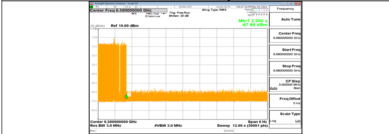
11BE320-CDD_Ant1_6425_High_6580_2
