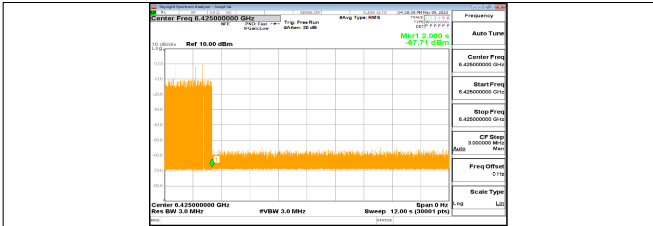
11BE320-CDD_Ant1_6425_Center_6425_1
