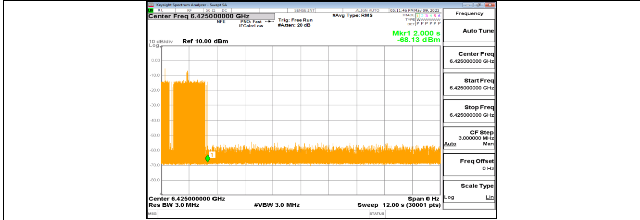
11BE320-CDD_Ant1_6425_Center_6425_6
