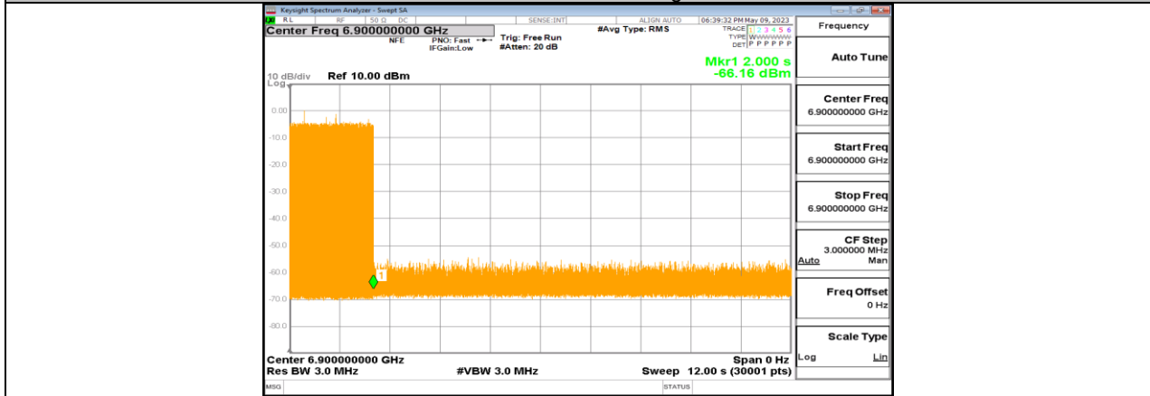
11BE320-CDD_Ant1_6745_High_6900_2
