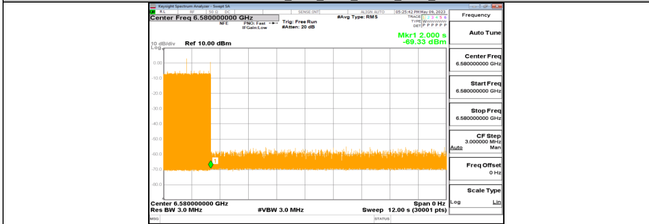
11BE320-CDD_Ant1_6425_High_6580_1
