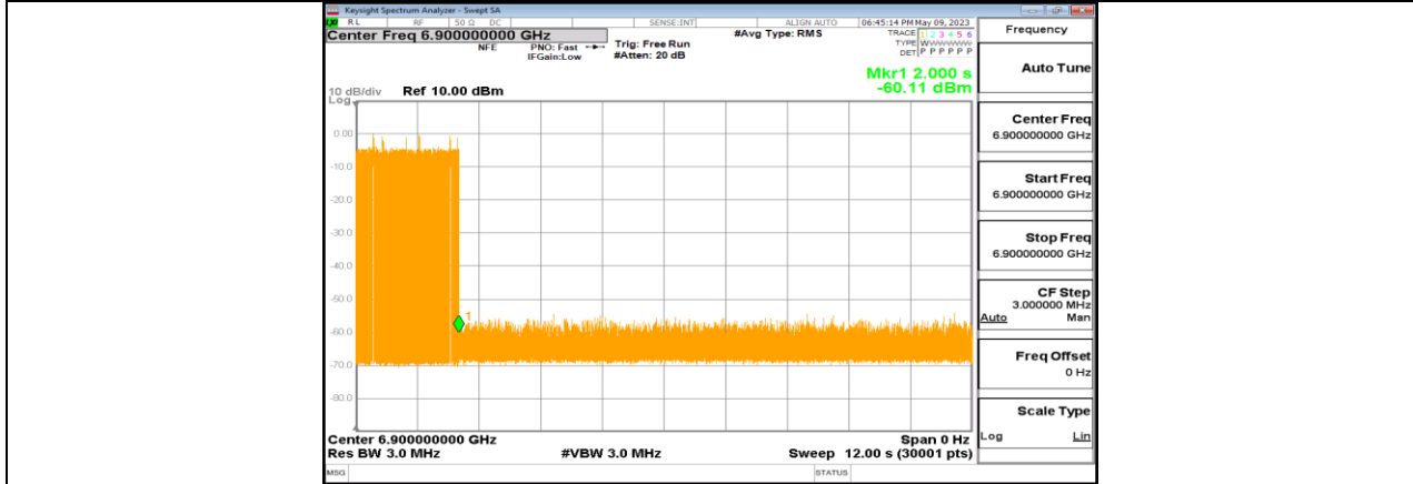
11BE320-CDD_Ant1_6745_High_6900_5
