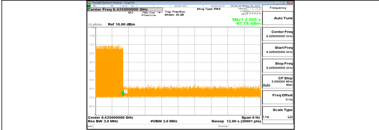
11BE320-CDD_Ant1_6425_Center_6425_3
