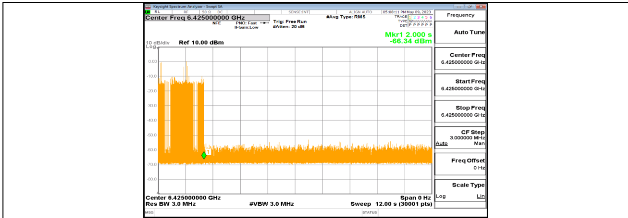
11BE320-CDD_Ant1_6425_Center_6425_4
