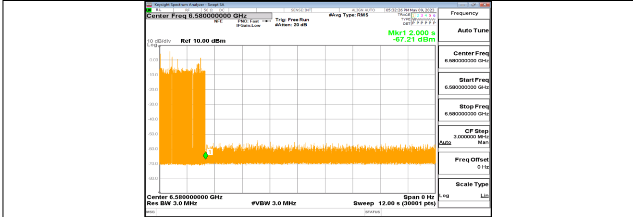
11BE320-CDD_Ant1_6425_High_6580_5
