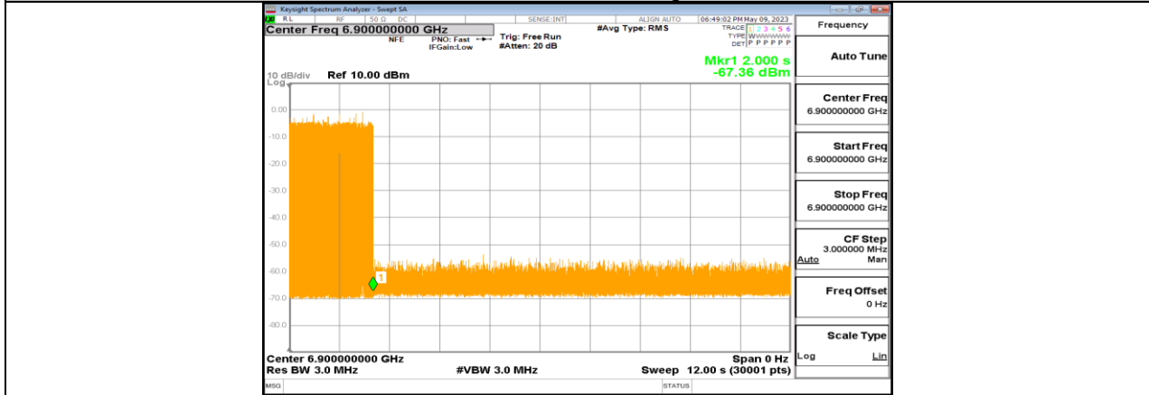
11BE320-CDD_Ant1_6745_High_6900_7
