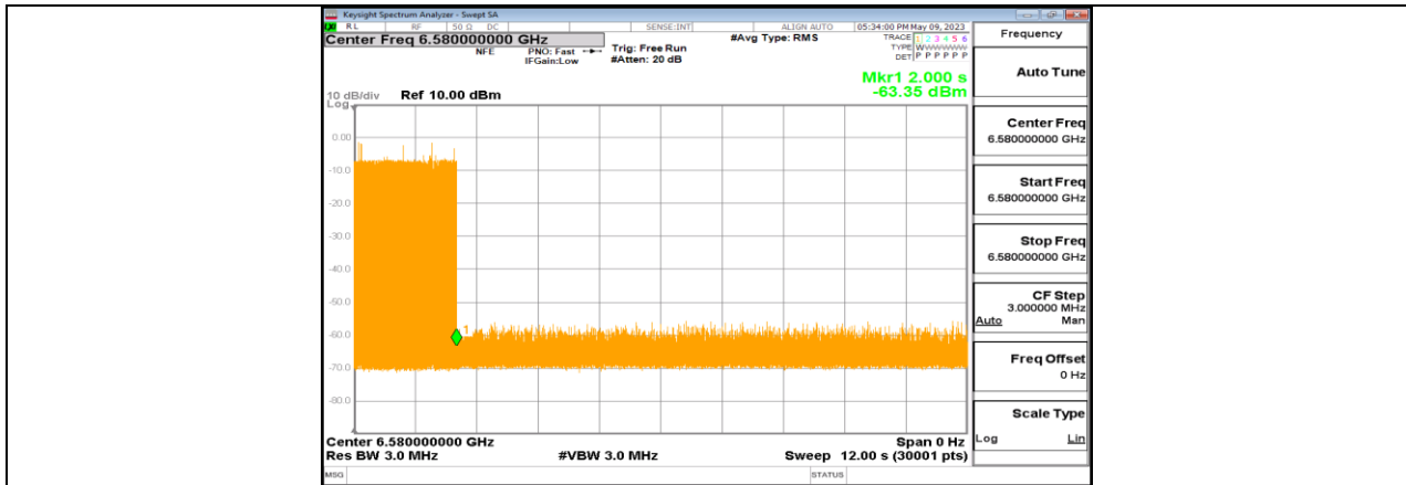
11BE320-CDD_Ant1_6425_High_6580_6
