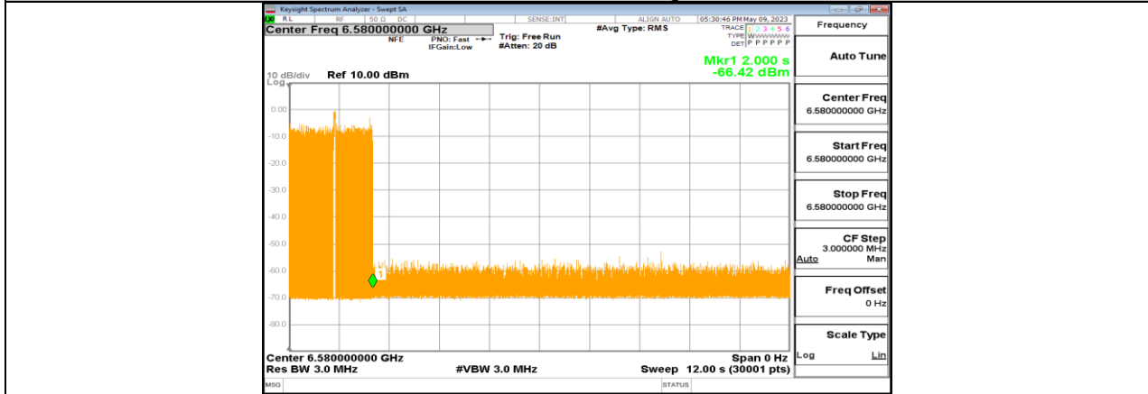
11BE320-CDD_Ant1_6425_High_6580_4
