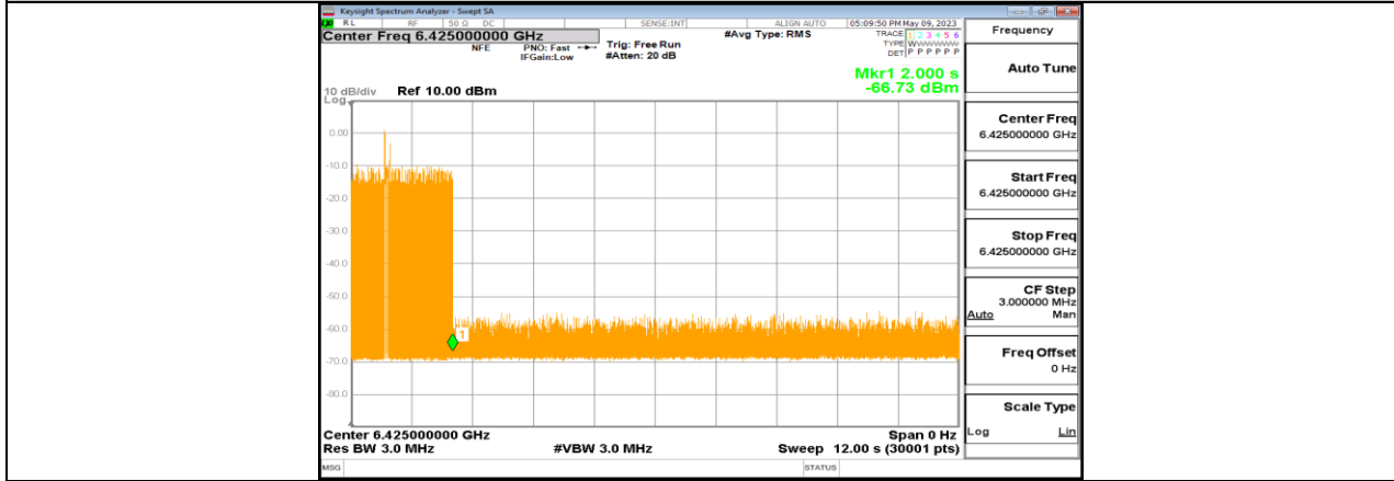
11BE320-CDD_Ant1_6425_Center_6425_5
