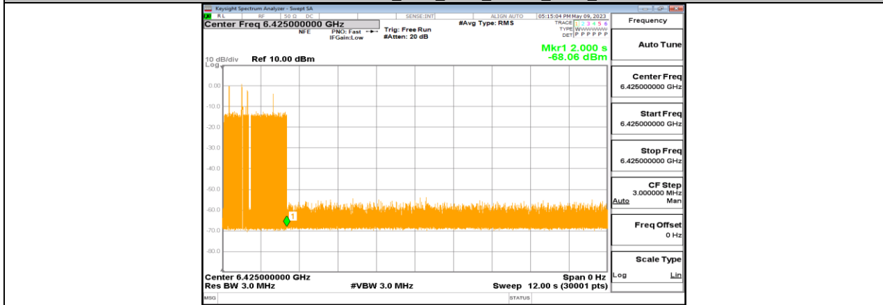
11BE320-CDD_Ant1_6425_Center_6425_8
