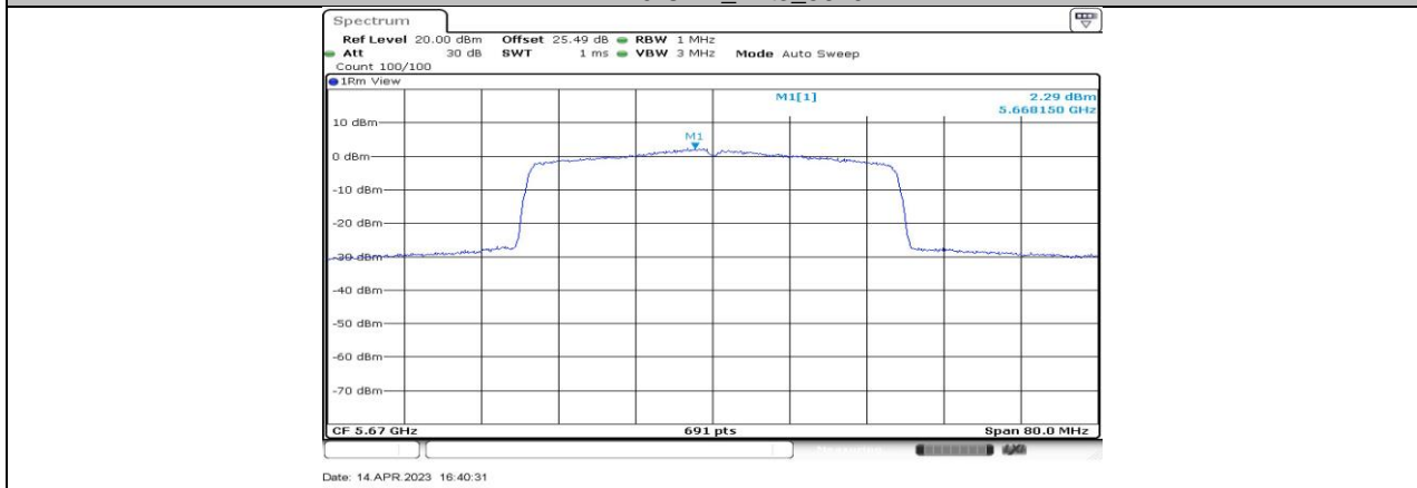
11BE40-CDD_Ant4_5670
