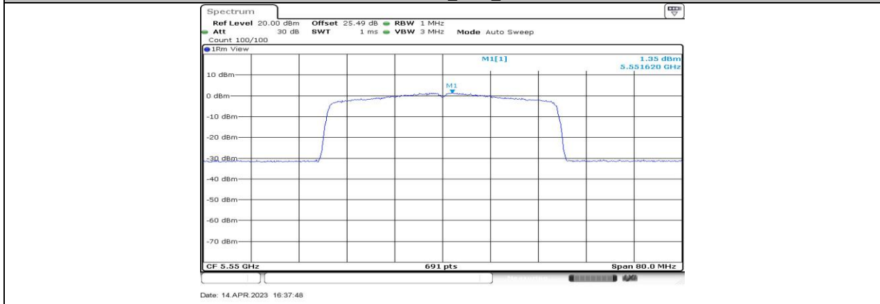
11BE40-CDD_Ant4_5550
