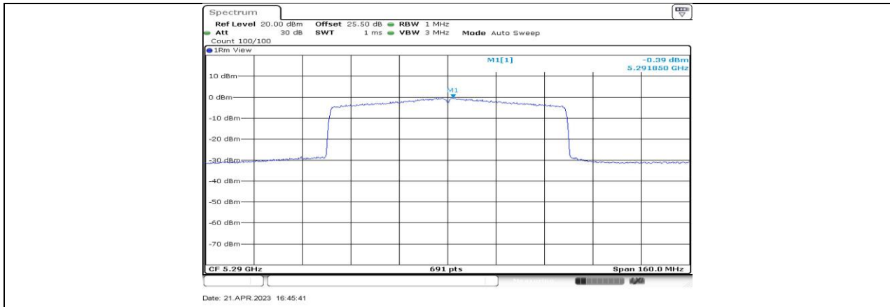
11BE80-CDD_Ant4_5290
