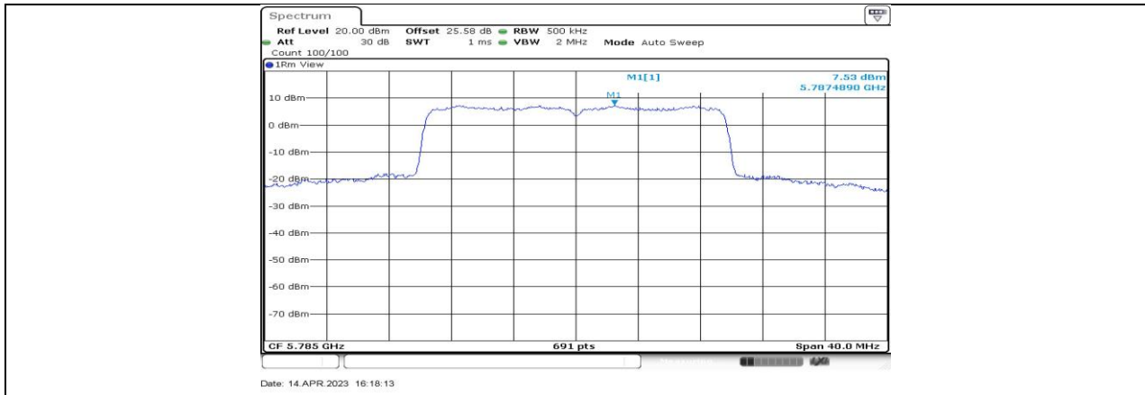
11BE20-CDD_Ant4_5785
