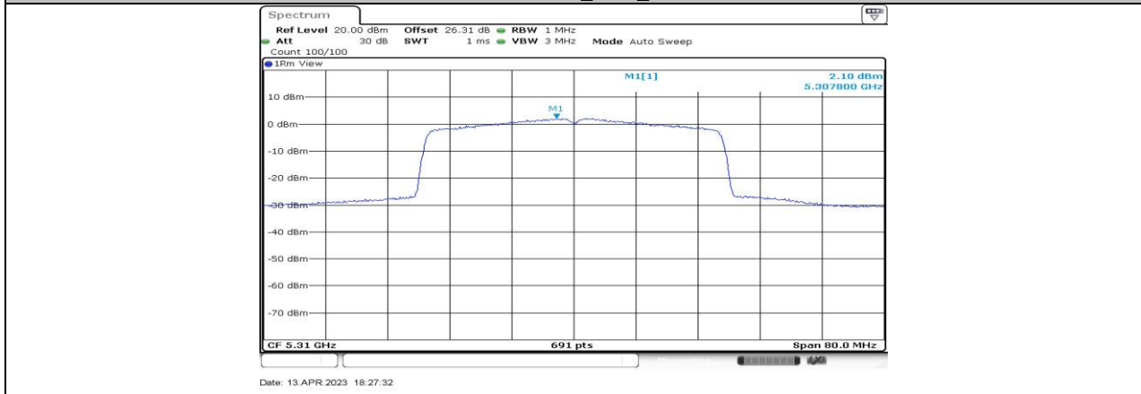
11AX40-CDD_Ant2_5310
