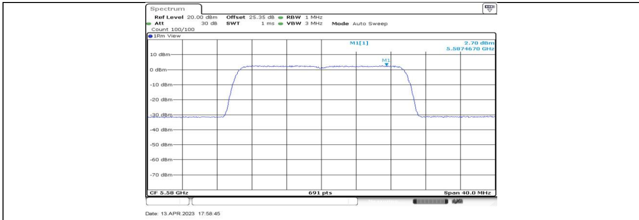
11AX20-CDD_Ant3_5580
