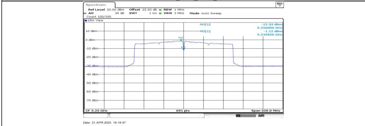
11AX160-CDD_Ant4_5250_UNII-1
