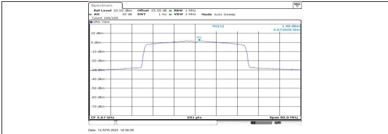
11AX40-CDD_Ant4_5670
