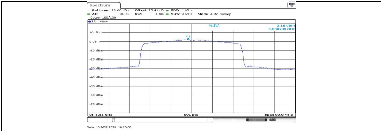
11AX40-CDD_Ant4_5310
