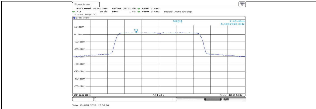
11AX20-CDD_Ant4_5500
