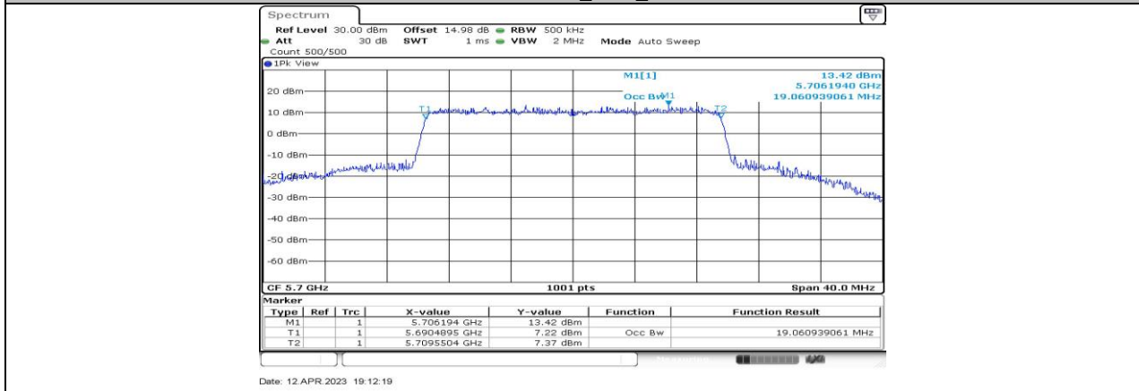
11AX20-CDD_Ant3_5700
