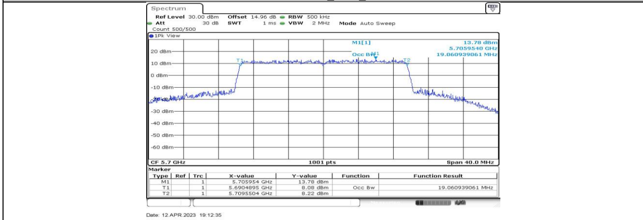
11AX20-CDD_Ant4_5700
