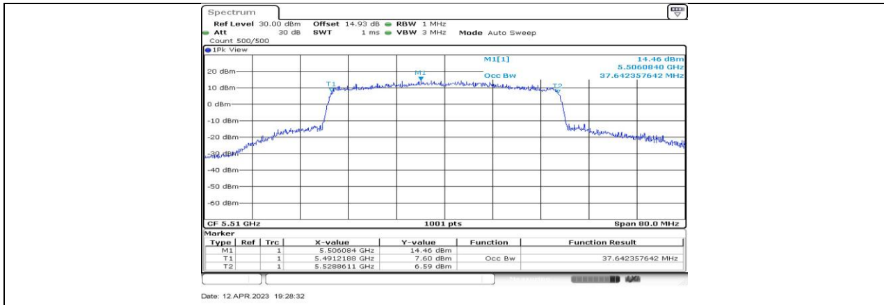
11AX40-CDD_Ant3_5510
