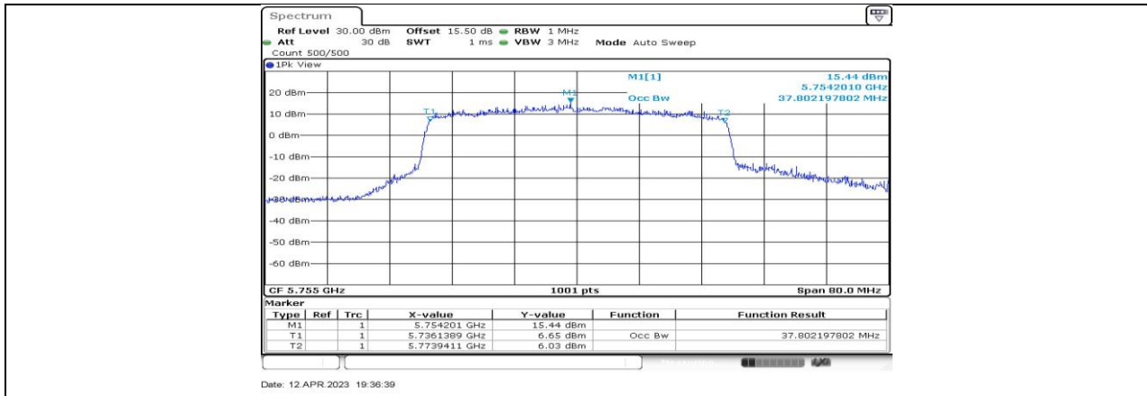
11AX40-CDD_Ant3_5755
