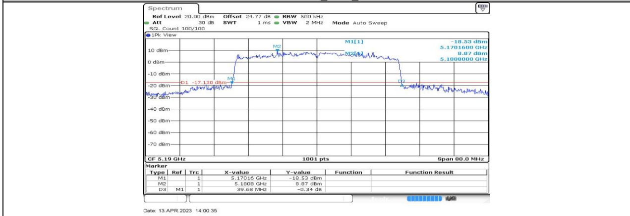
11BE40-CDD_Ant4_5190
