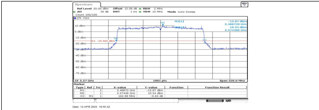
11AX160-CDD_Ant4_5570
