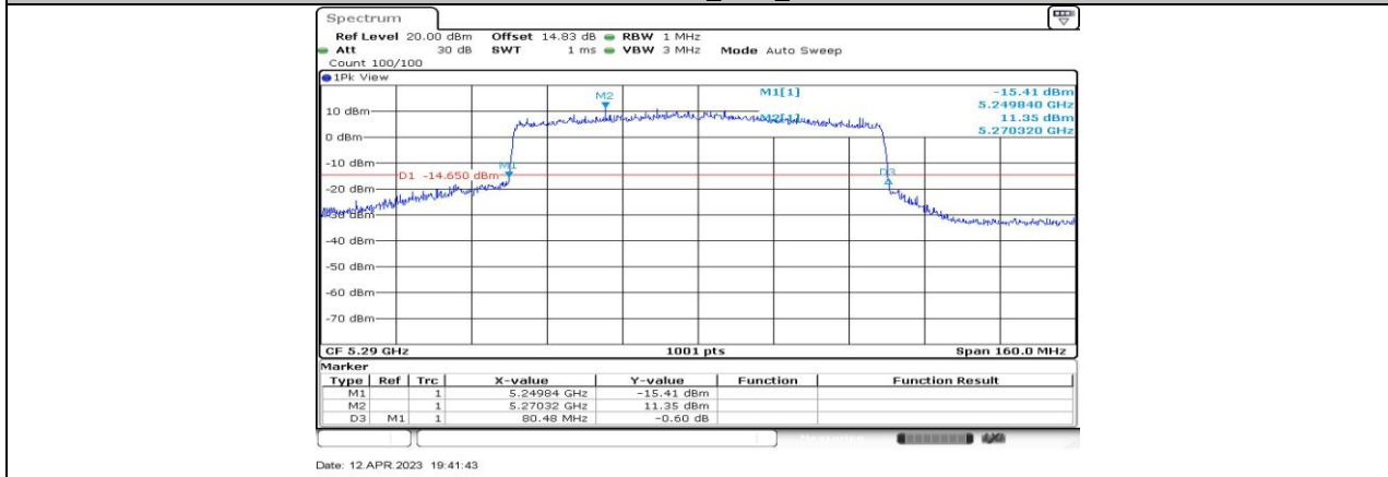
11AX80-CDD_Ant4_5290
