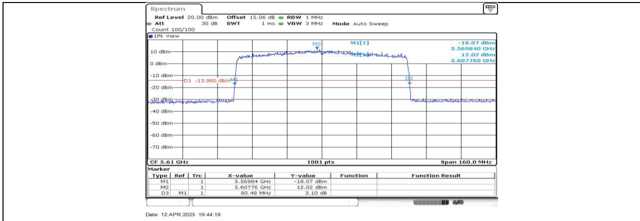
11AX80-CDD_Ant4_5610
