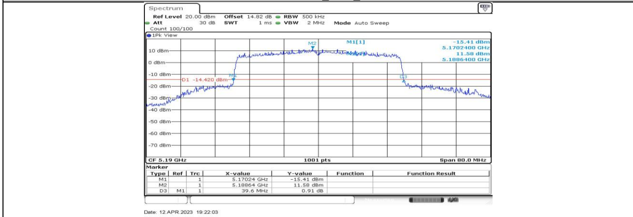
11AX40-CDD_Ant3_5190
