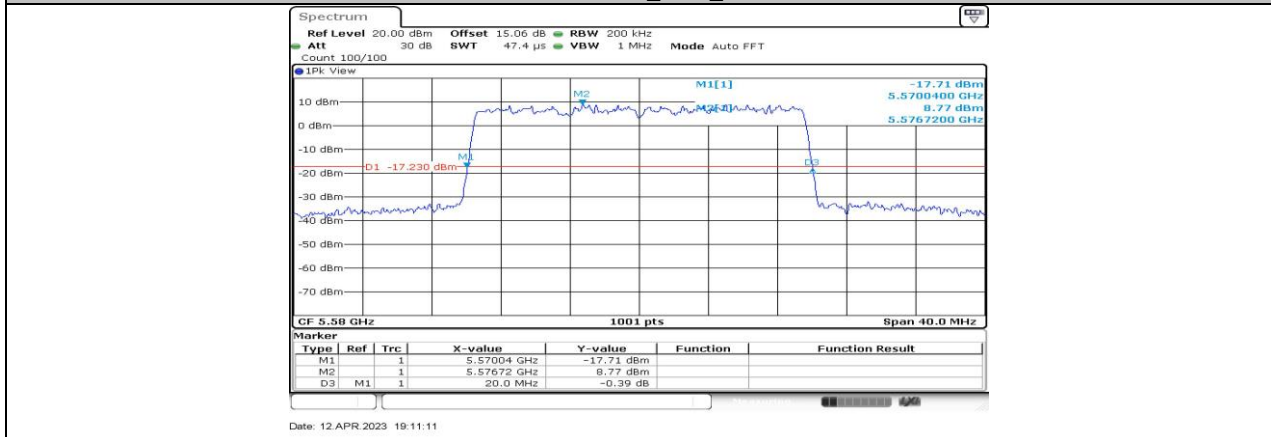
11AX20-CDD_Ant4_5580
