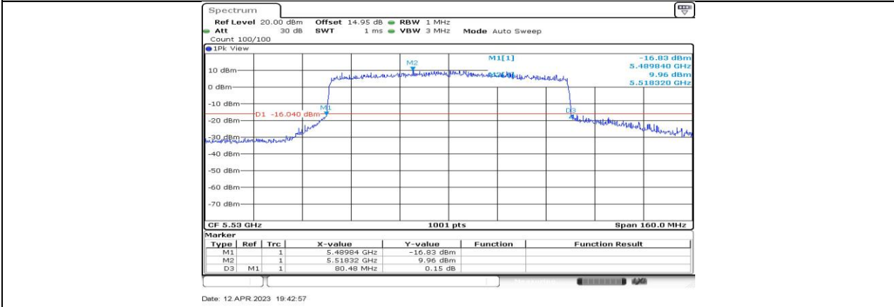
11AX80-CDD_Ant4_5530
