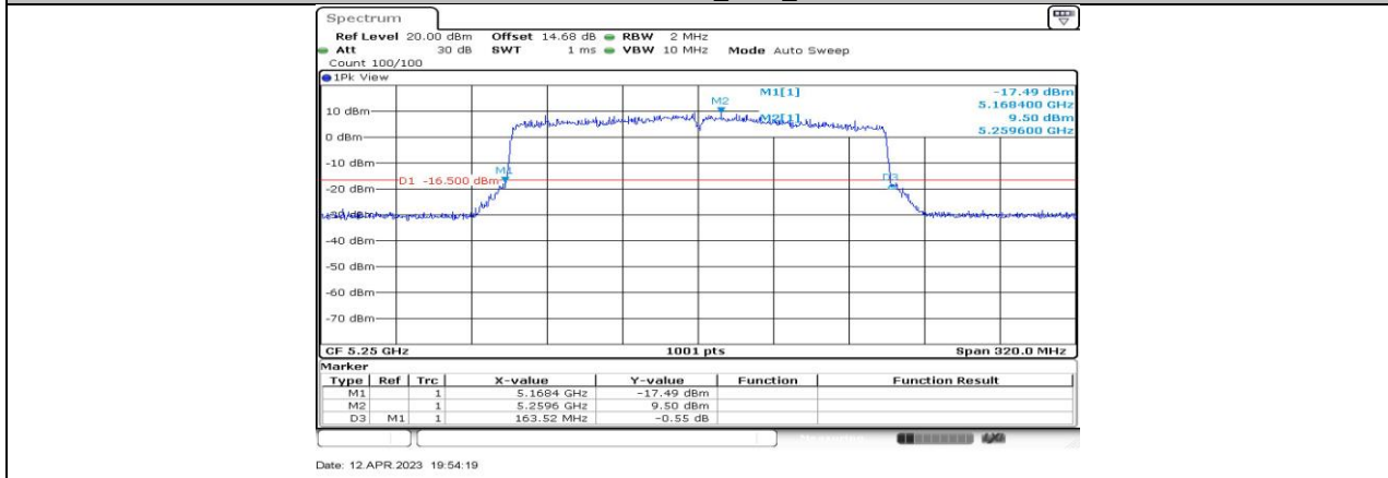
11AX160-CDD_Ant4_5250
