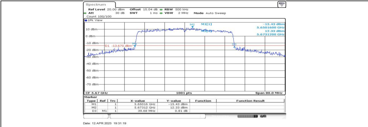
11AX40-CDD_Ant4_5670
