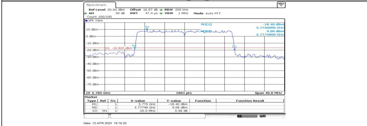
11AX20-CDD_Ant2_5785
