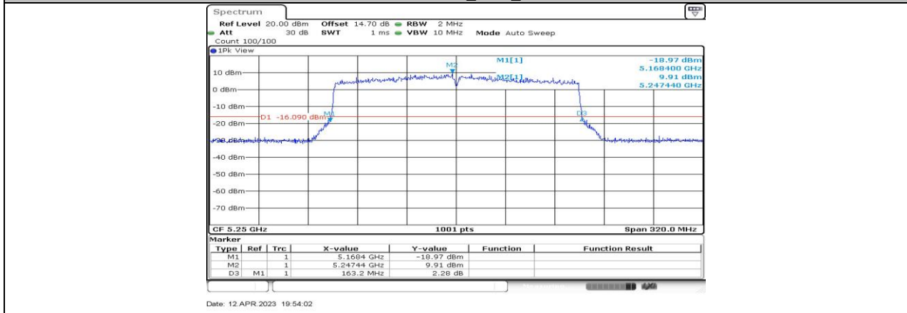
11AX160-CDD_Ant3_5250
