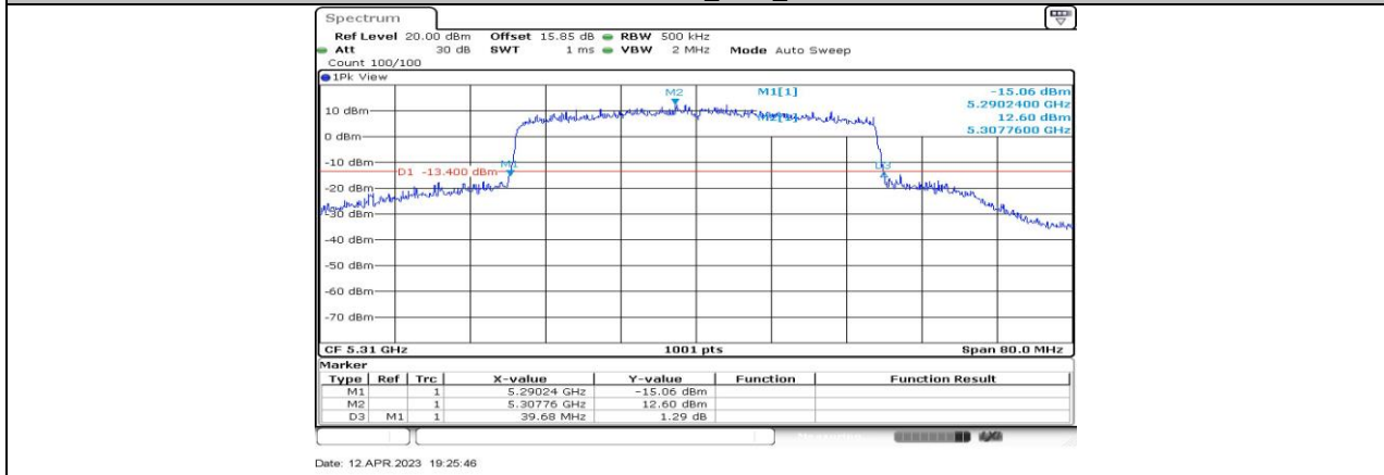
11AX40-CDD_Ant2_5310
