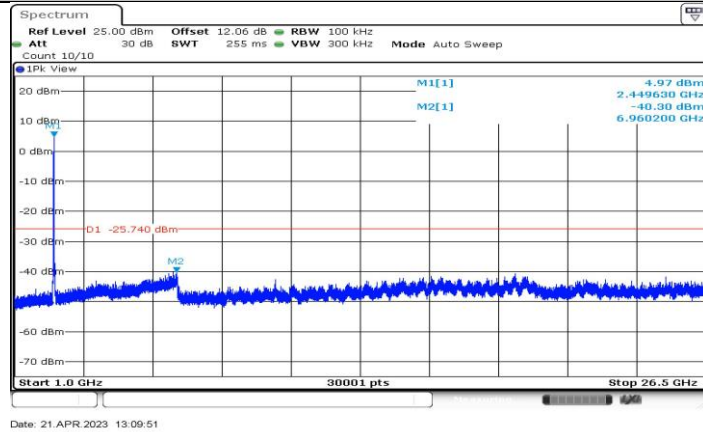
11AX40-CDD_Ant1_2447_1000~26500
