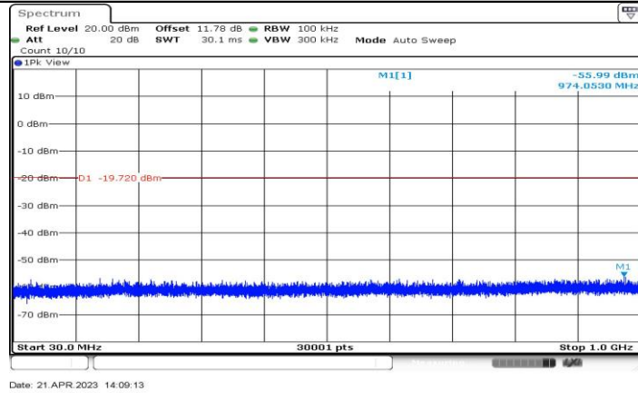
11BE20-CDD_Ant3_2412_30~1000
