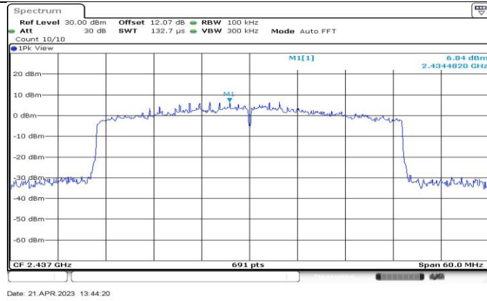
11AX40-CDD_Ant1_2437_0~Reference
