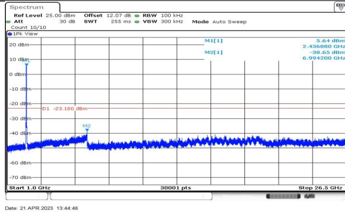
11AX40-CDD_Ant1_2437_1000~26500
