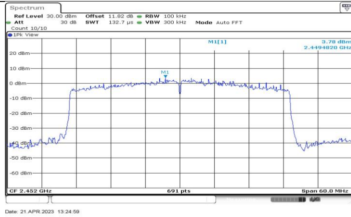
11AX40-CDD_Ant4_2452_0~Reference
