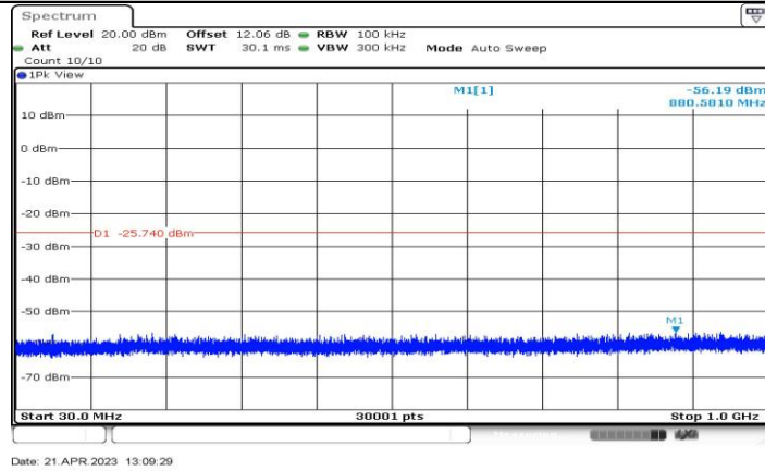
11AX40-CDD_Ant1_2447_30~1000
