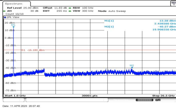
11BE20-CDD_Ant3_2437_1000~26500
