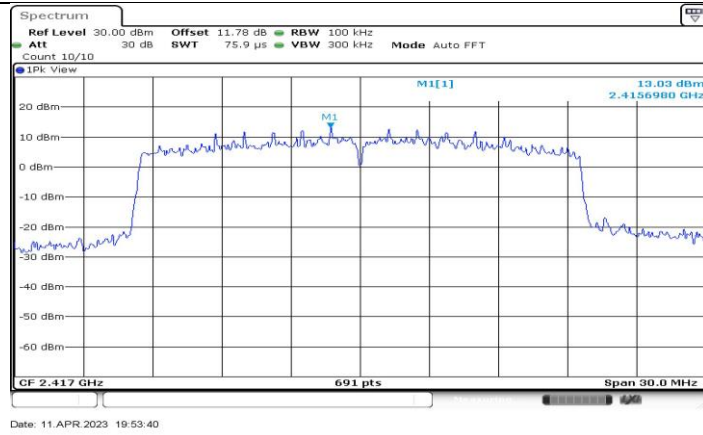
11BE20-CDD_Ant3_2417_0~Reference
