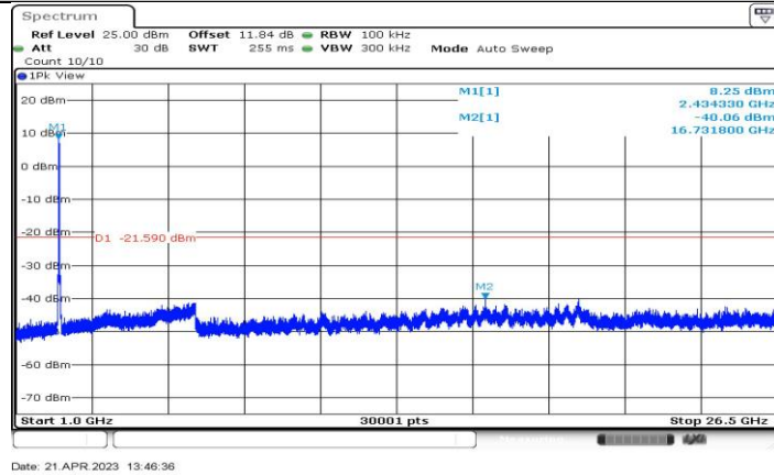
11AX40-CDD_Ant4_2437_1000~26500
