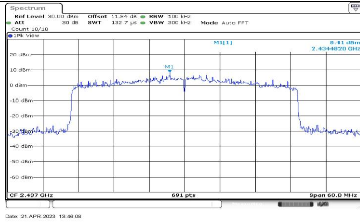
11AX40-CDD_Ant4_2437_0~Reference
