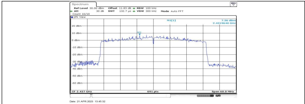
11AX40-CDD_Ant3_2437_0~Reference
