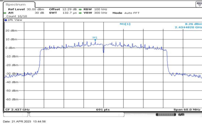
11AX40-CDD_Ant2_2437_0~Reference
