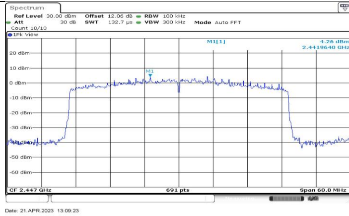
11AX40-CDD_Ant1_2447_0~Reference
