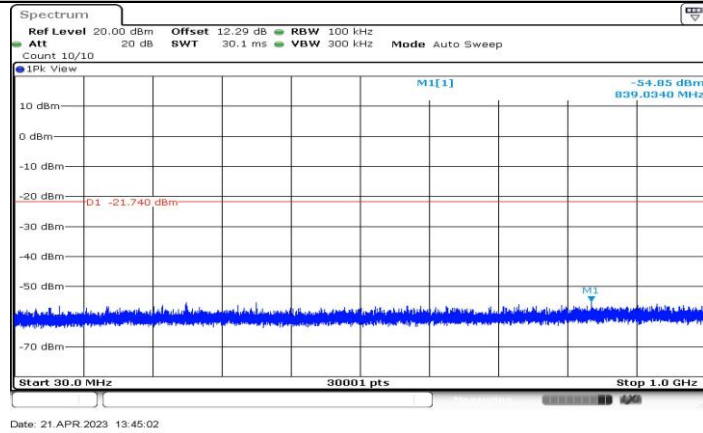
11AX40-CDD_Ant2_2437_30~1000
