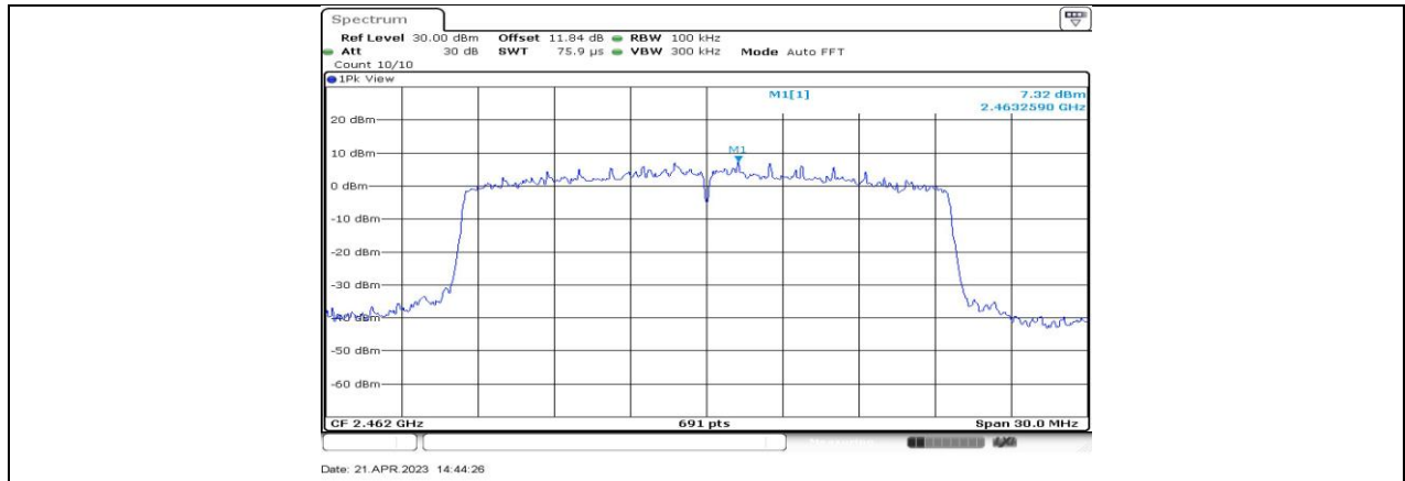
11BE20-CDD_Ant3_2462_0~Reference
