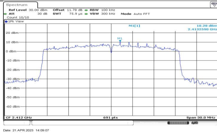
11BE20-CDD_Ant3_2412_0~Reference
