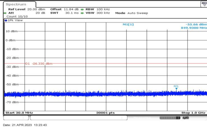
11AX40-CDD_Ant3_2452_30~1000
