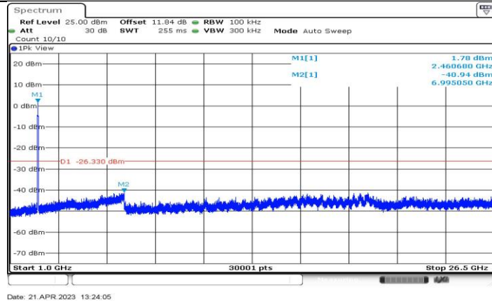
11AX40-CDD_Ant3_2452_1000~26500
