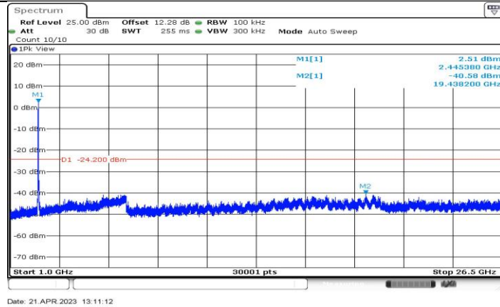
11AX40-CDD_Ant2_2447_1000~26500
