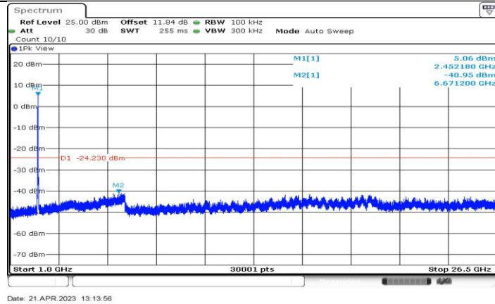
11AX40-CDD_Ant4_2447_1000~26500
