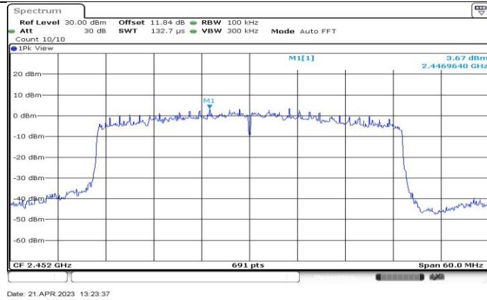
11AX40-CDD_Ant3_2452_0~Reference
