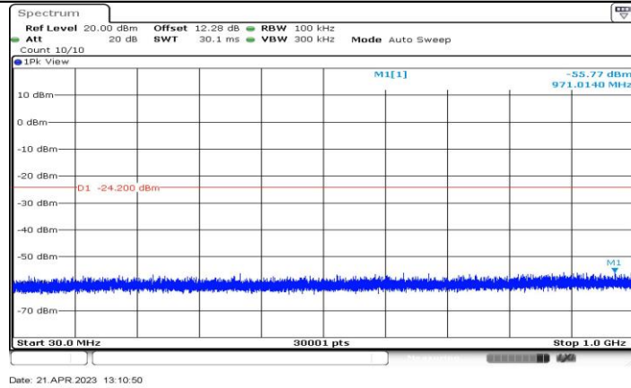
11AX40-CDD_Ant2_2447_30~1000
