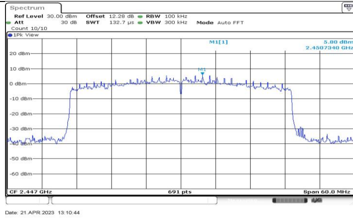
11AX40-CDD_Ant2_2447_0~Reference
