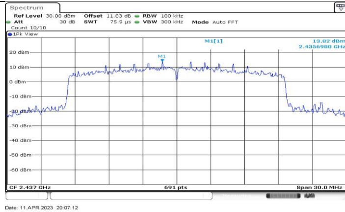
11BE20-CDD_Ant3_2437_0~Reference
