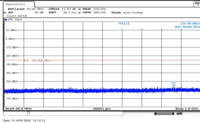
11AX40-CDD_Ant3_2447_30~1000
