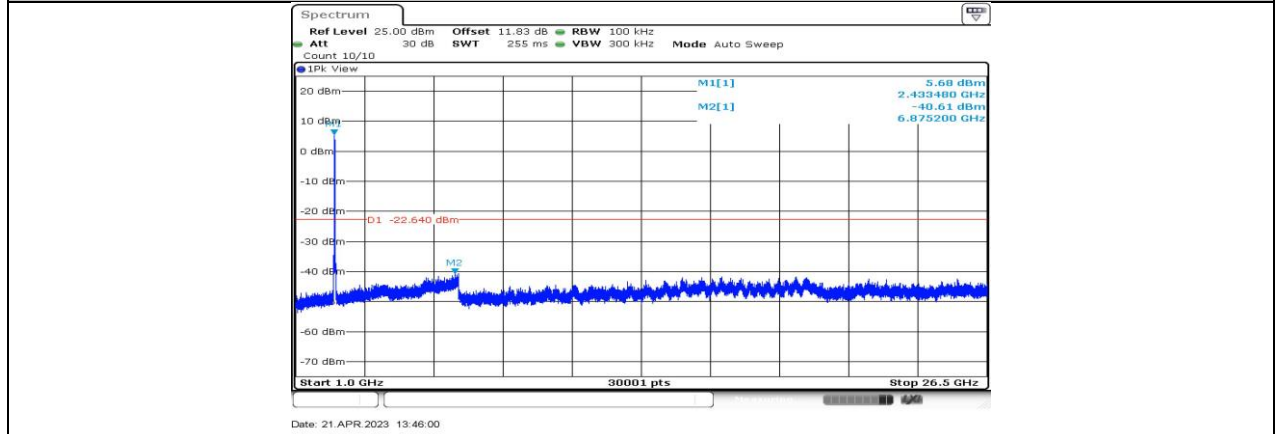
11AX40-CDD_Ant3_2437_1000~26500
