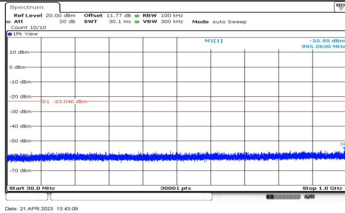
11AX40-CDD_Ant4_2427_30~1000
