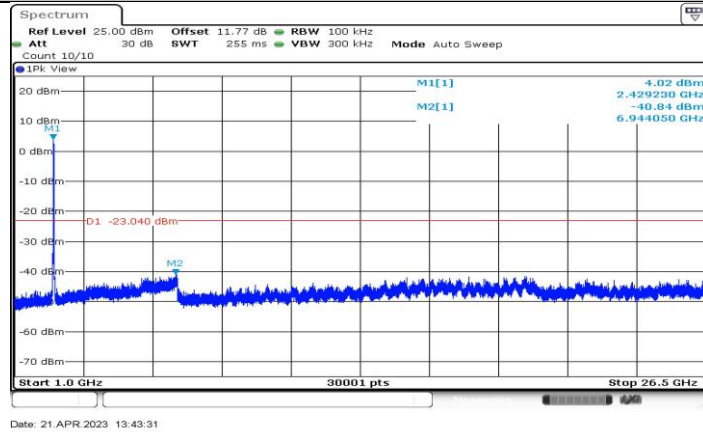
11AX40-CDD_Ant4_2427_1000~26500
