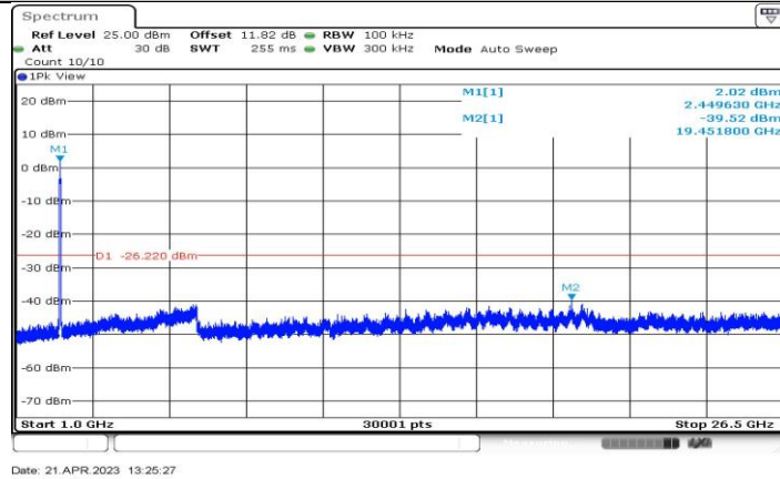
11AX40-CDD_Ant4_2452_1000~26500
