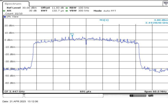
11AX40-CDD_Ant3_2447_0~Reference
