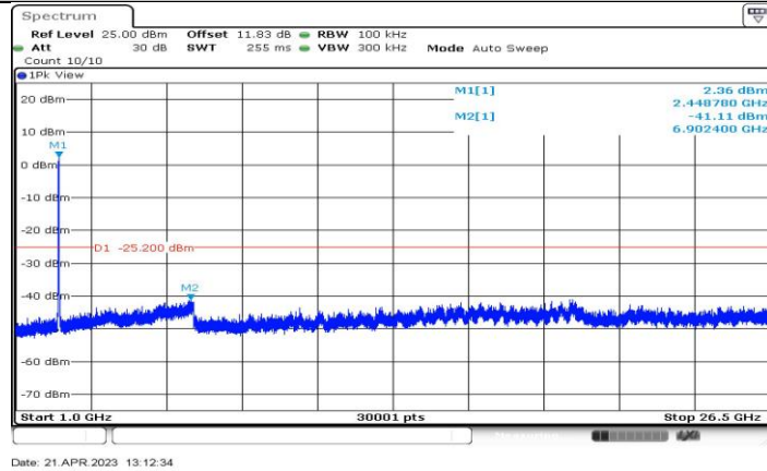
11AX40-CDD_Ant3_2447_1000~26500
