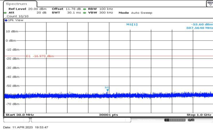
11BE20-CDD_Ant3_2417_30~1000
