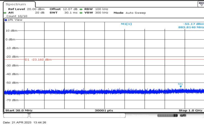
11AX40-CDD_Ant1_2437_30~1000
