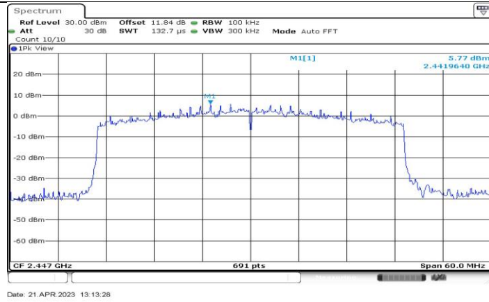
11AX40-CDD_Ant4_2447_0~Reference
