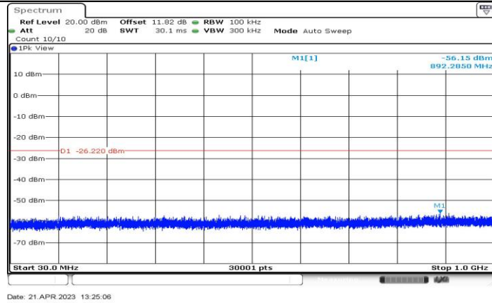
11AX40-CDD_Ant4_2452_30~1000
