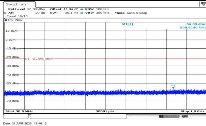
11AX40-CDD_Ant4_2437_30~1000
