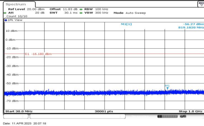
11BE20-CDD_Ant3_2437_30~1000
