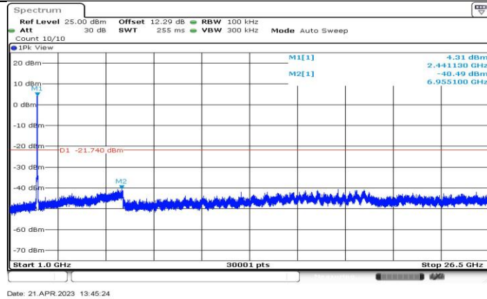
11AX40-CDD_Ant2_2437_1000~26500
