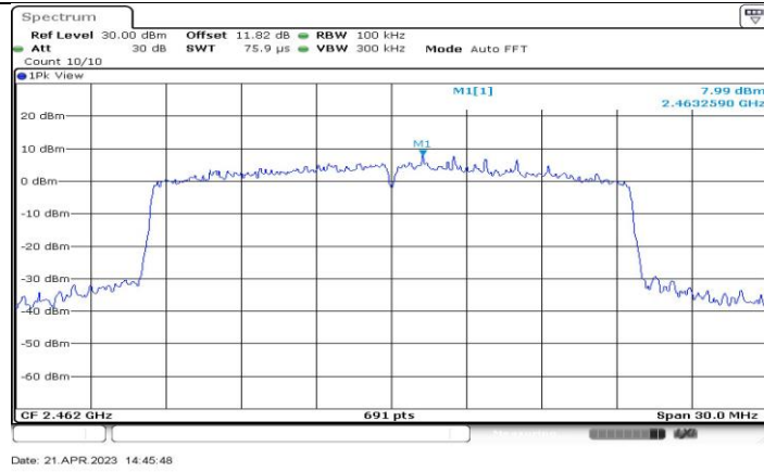
11BE20-CDD_Ant4_2462_0~Reference
