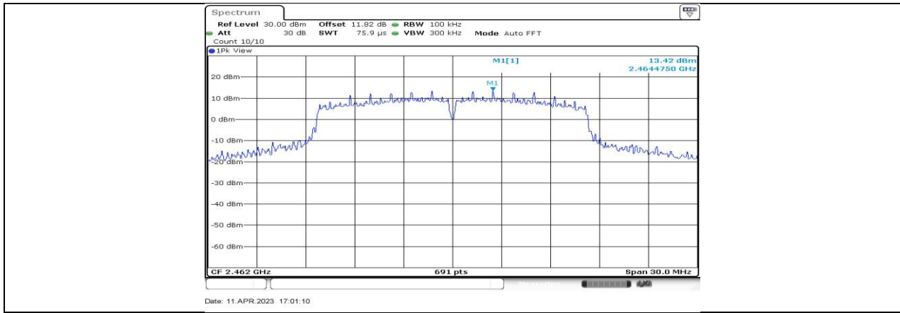
11G-CDD_Ant4_2462_0~Reference
