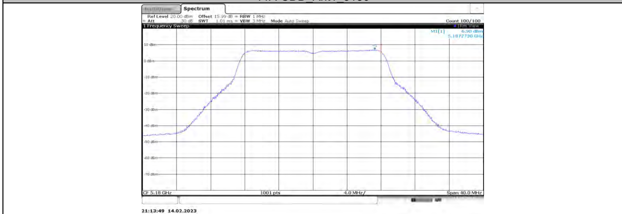
11A-CDD Ant2 5180
