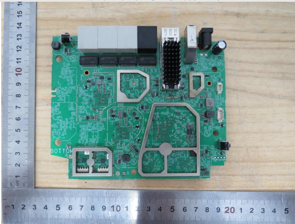
Internal View of EUT-13-Deco BE79
