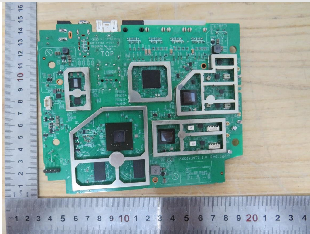
Internal View of EUT-12-Deco BE79
