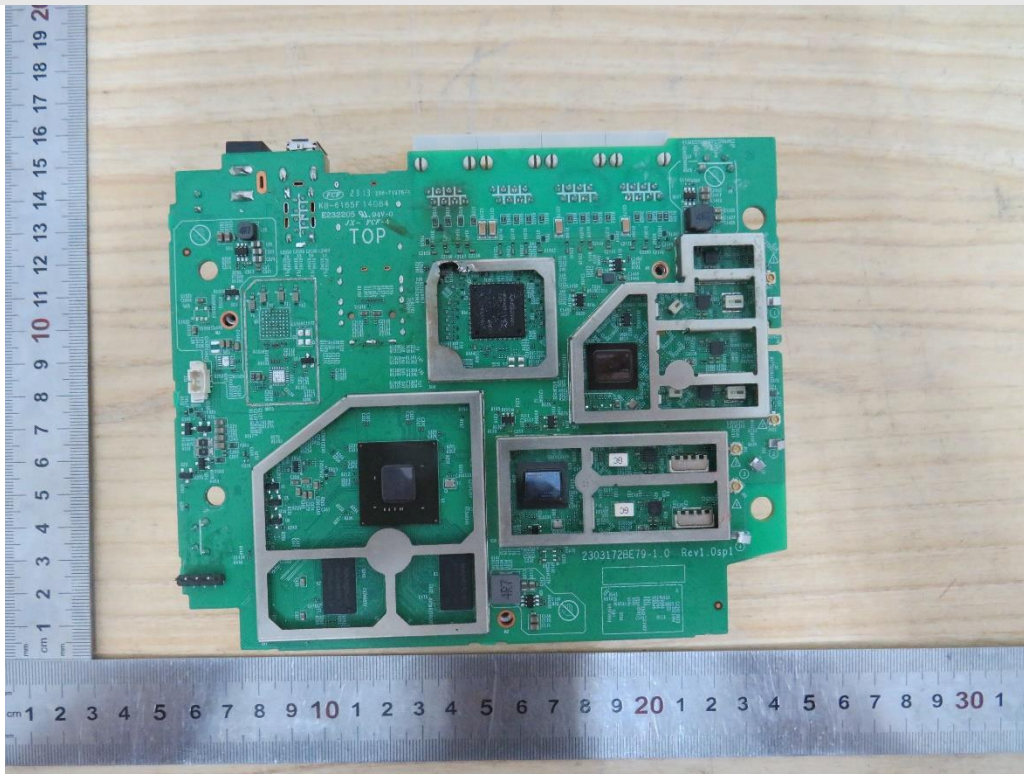
Internal View of EUT-13-Deco BE16000
