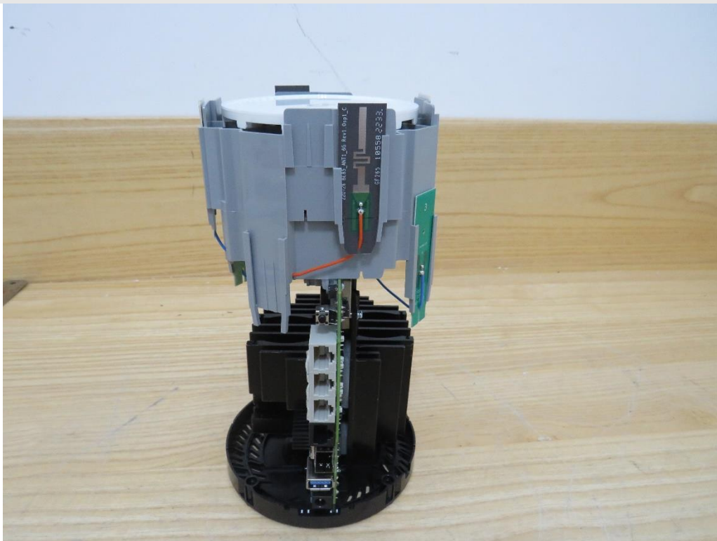
Internal View of EUT-2-Deco BE79
