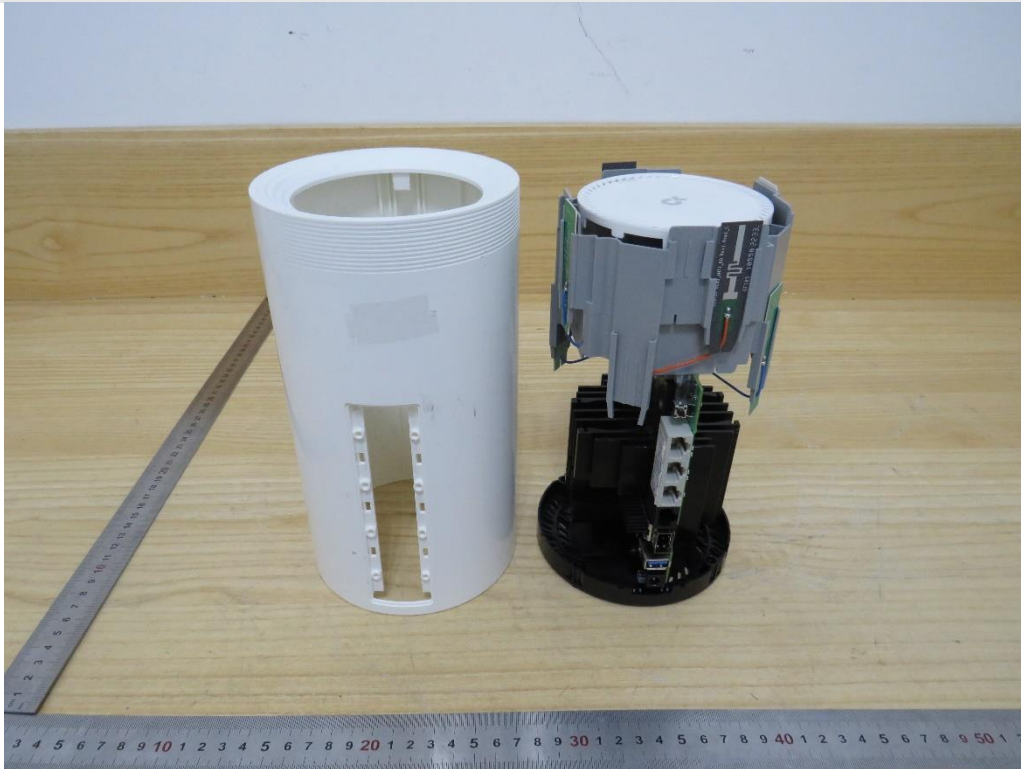
Internal View of EUT-1-Deco BE79
