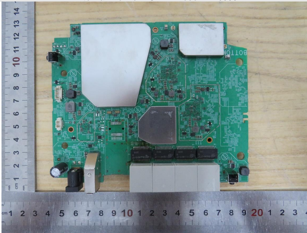
Internal View of EUT-11-Deco BE16000
