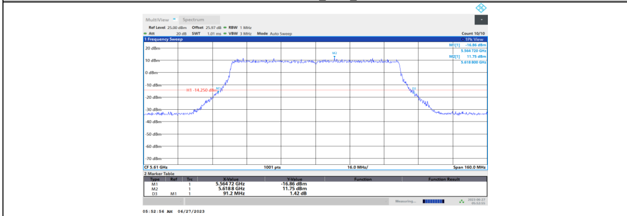
11AX80-CDD_Ant6_5610
