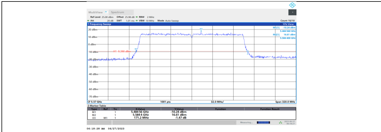
11AX160-CDD_Ant6_5570
