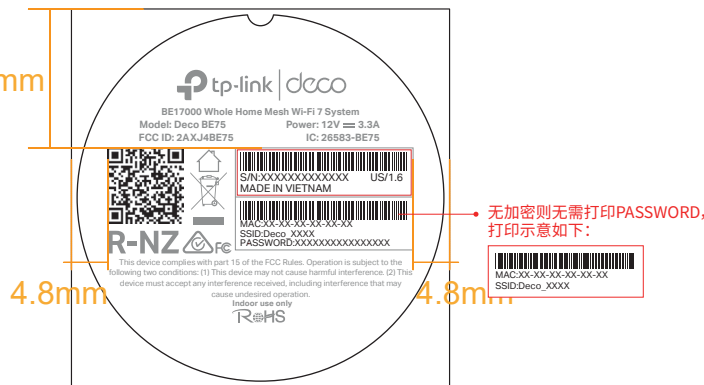
圆: 48.5*48.5mm ±0.2 外框方形: 50*50mm ±0.2
