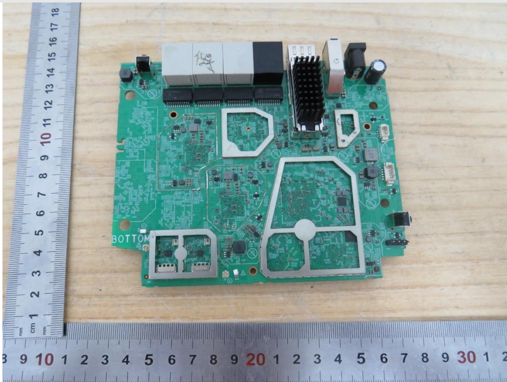
Internal View of EUT-12-Deco BE75
