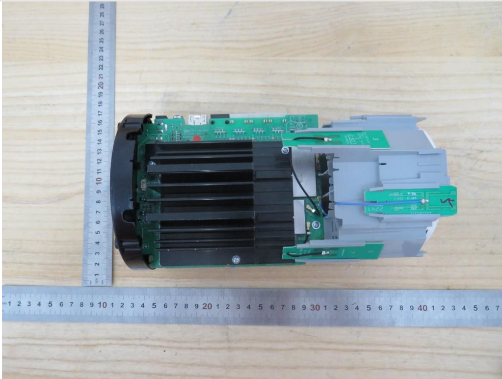
Internal View of EUT-10-Deco BE75
