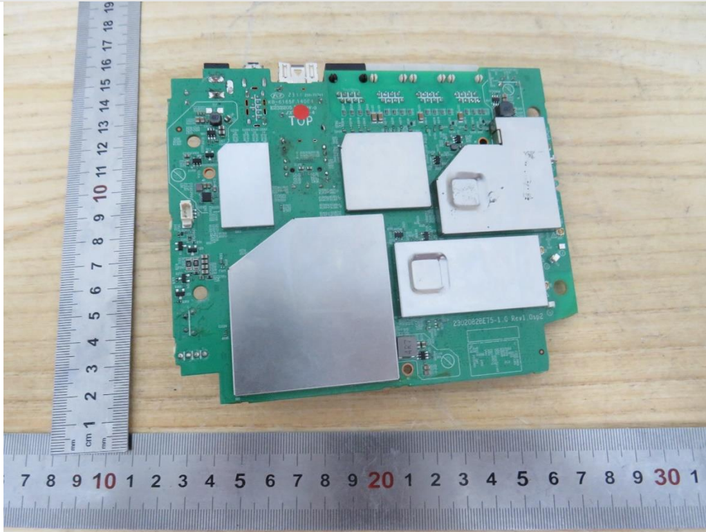
Internal View of EUT-13-Deco BE75
