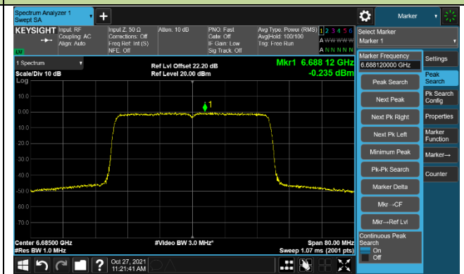
Channel 147 (6685MHz)
