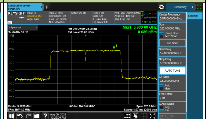
Channel 114 (5570MHz)
