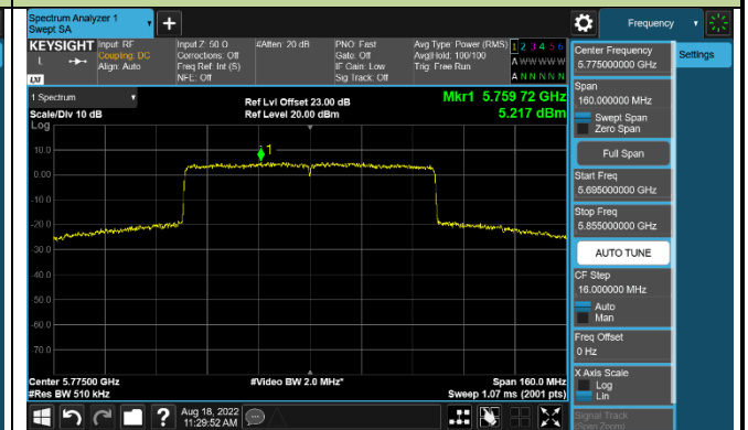
Channel 155 (5775MHz)
