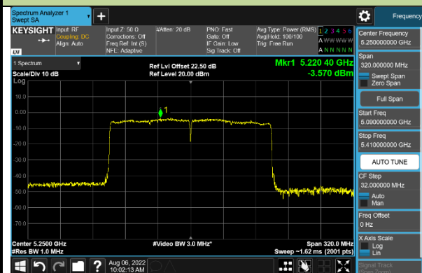
Channel 50 (5250MHz)
