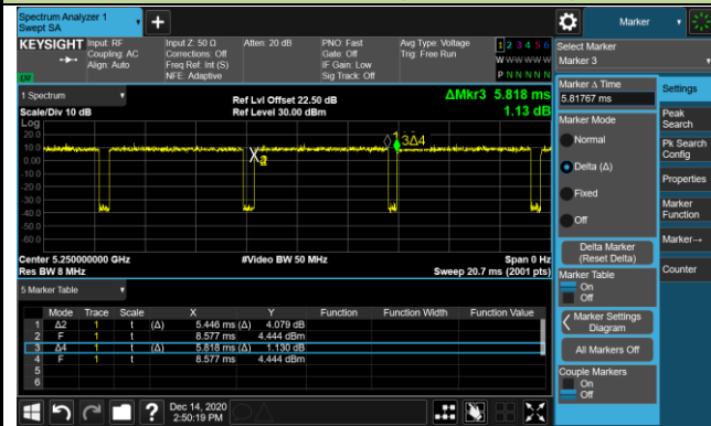
802.11ax-HE160(T=5.446ms)
