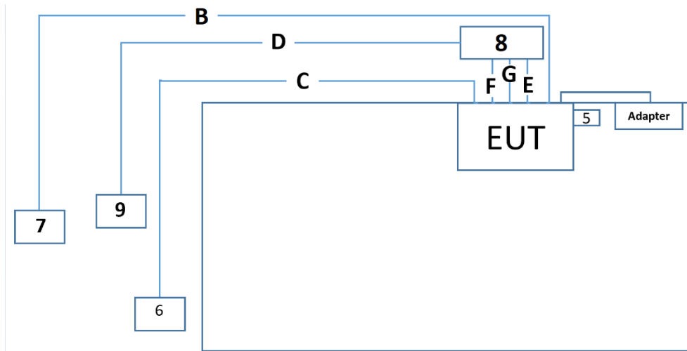
Connection Diagram- AC Conducted Emissions
