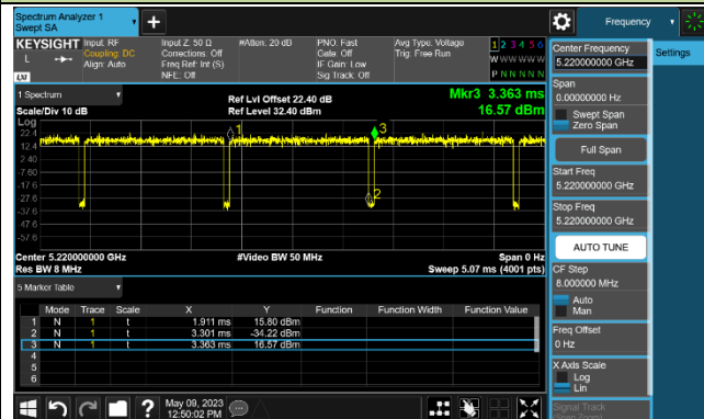
802.11ac-VHT40
