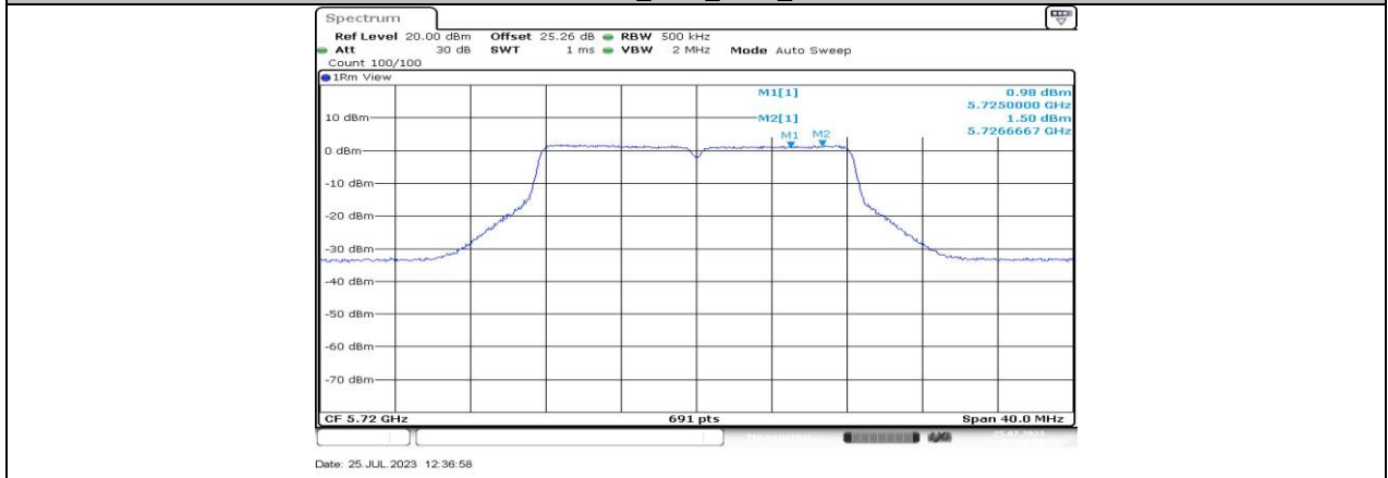
11A-CDD_Ant4_5720_UNII-3
