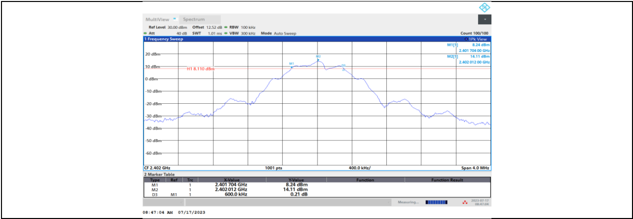
BLE_125 kbps_Ant1_2402
