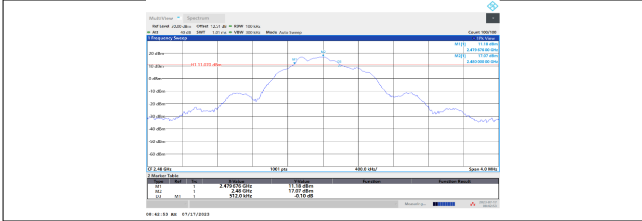
BLE_1 Mbps_Ant1_2480
