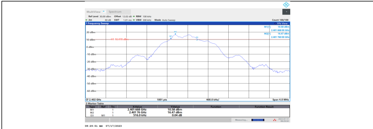
BLE_1 Mbps_Ant1_2402
