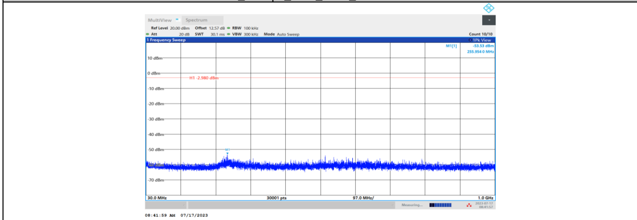
BLE_1 Mbps_Ant1_2440_30~1000
