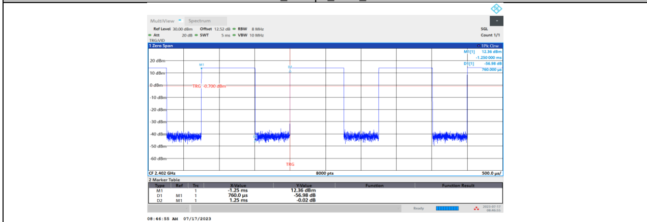
BLE_125 kbps_Ant1_2402
