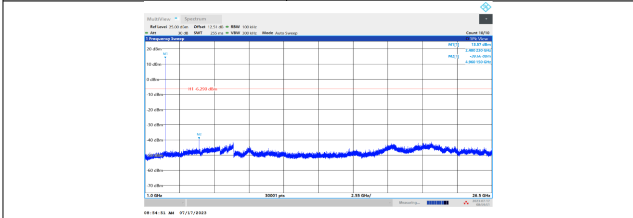
BLE_125 kbps_Ant1_2480_1000~26500
