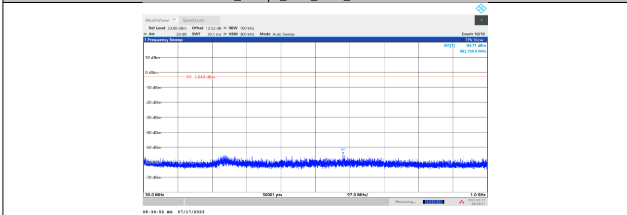
BLE_1 Mbps_Ant1_2402_30~1000
