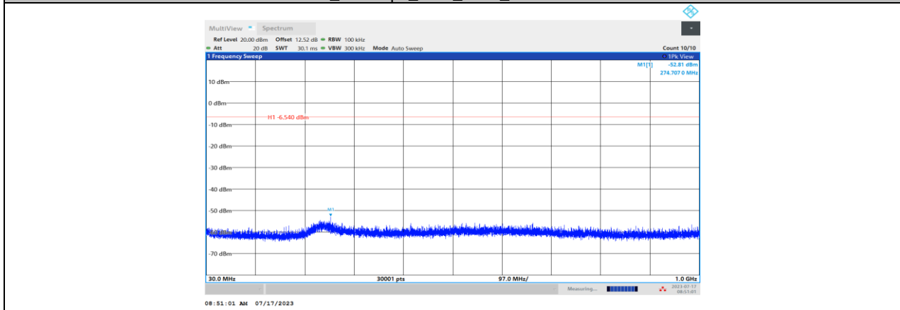
BLE_125 kbps_Ant1_2402_30~1000
