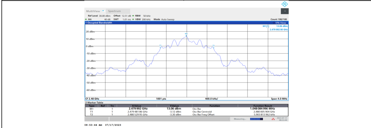
BLE_125 kbps_Ant1_2480
