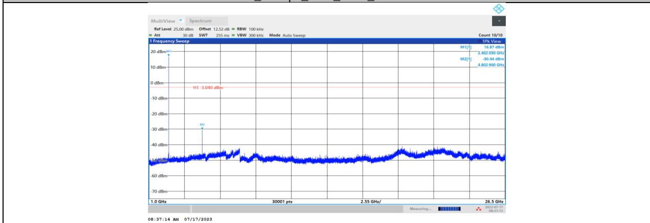
BLE_1 Mbps_Ant1_2402_1000~26500
