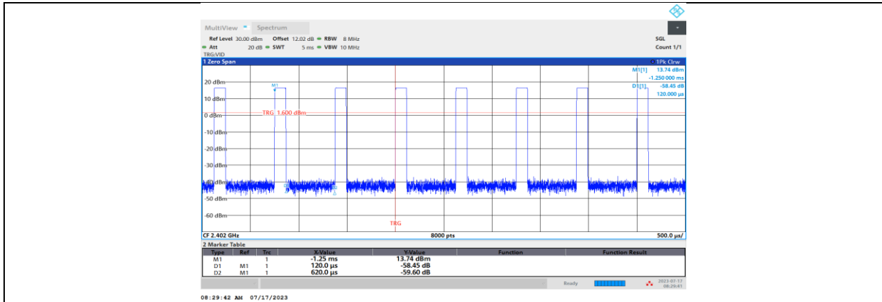
BLE_1 Mbps_Ant1_2402
