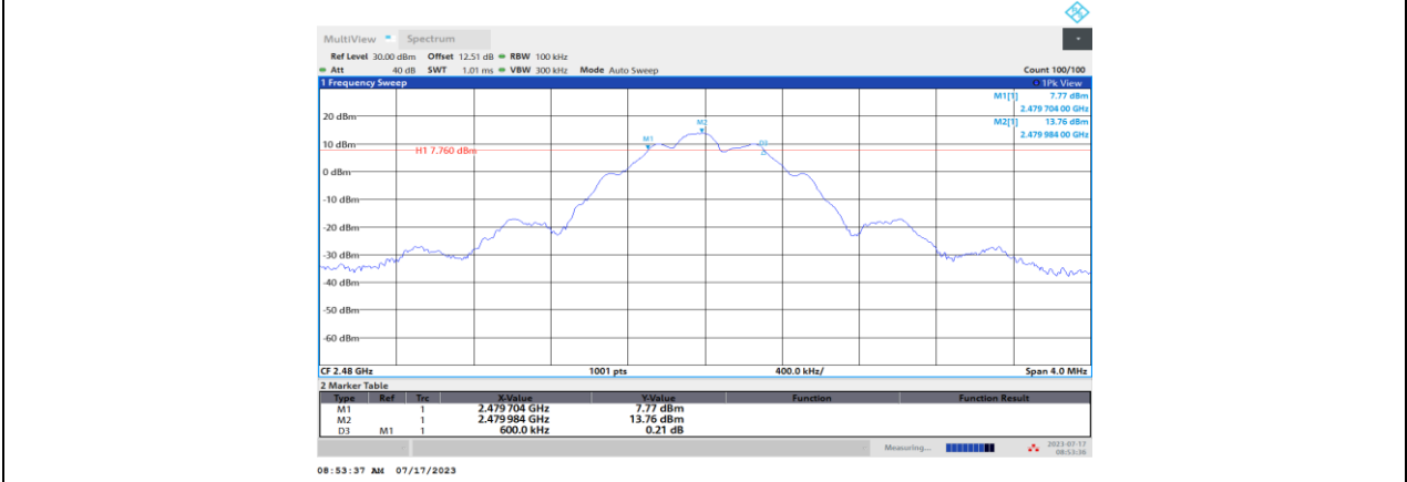
BLE_125 kbps_Ant1_2480
