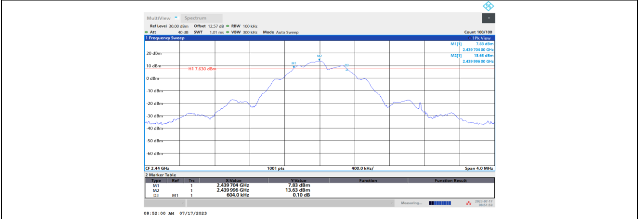
BLE_125 kbps_Ant1_2440
