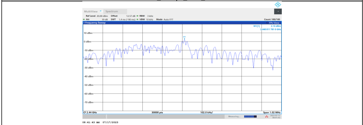
BLE_1 Mbps_Ant1_2440
