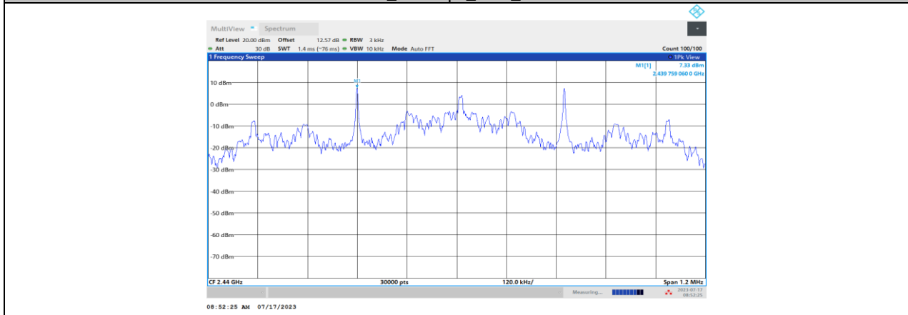
BLE_125 kbps_Ant1_2440
