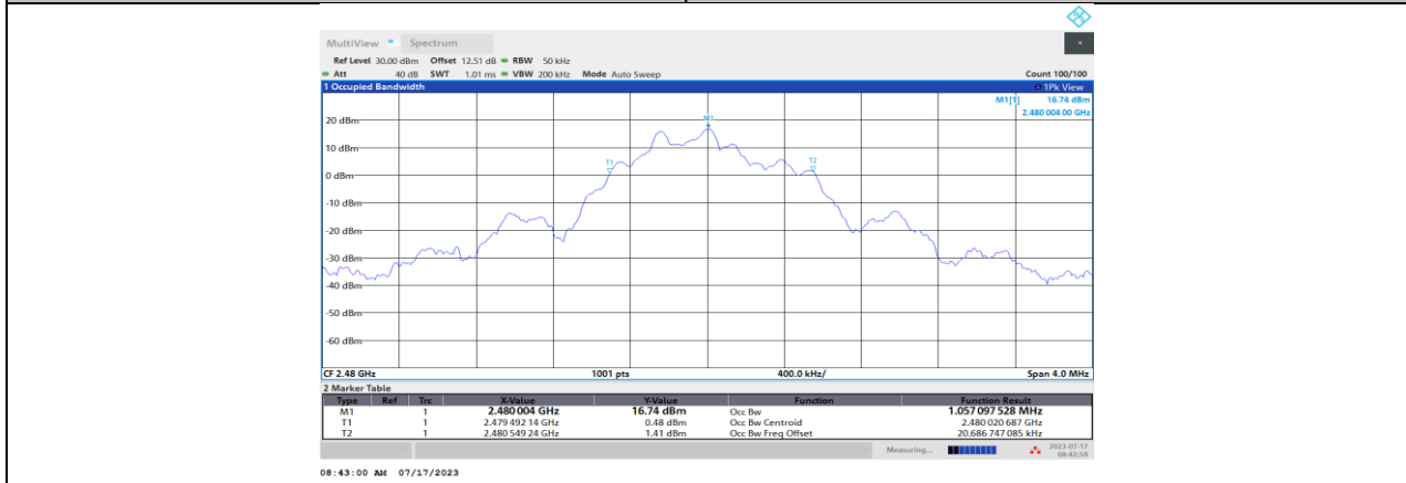
BLE_1 Mbps_Ant1_2480
