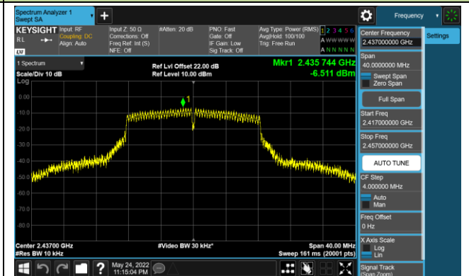
Channel 06 (2437MHz)
