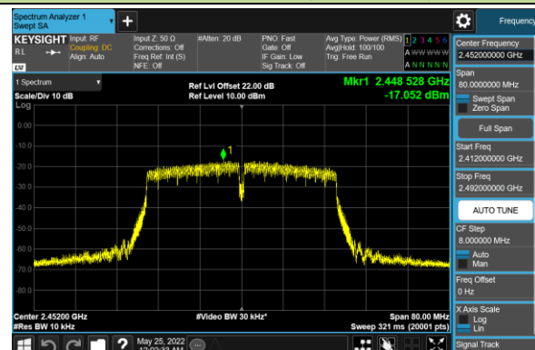
Channel 09 (2452MHz)
