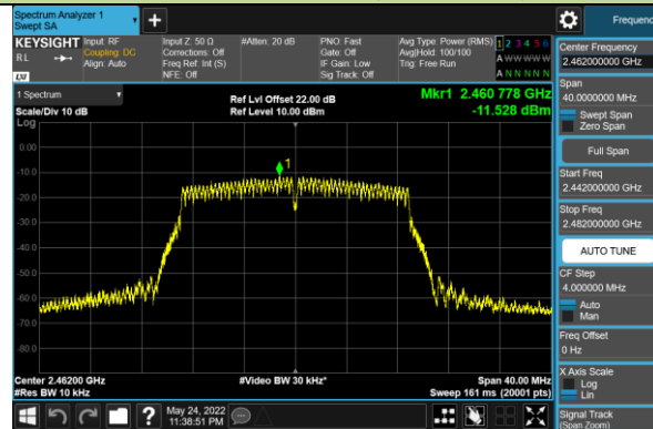
Channel 11 (2462MHz)
