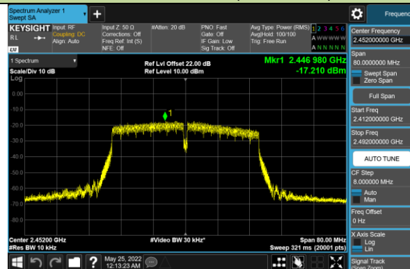
Channel 09 (2452MHz)
