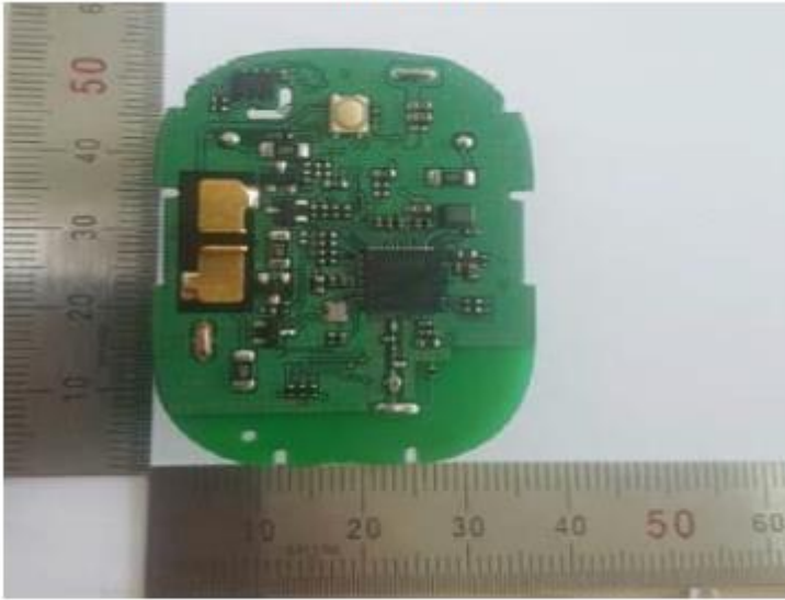
< Board bottom >
