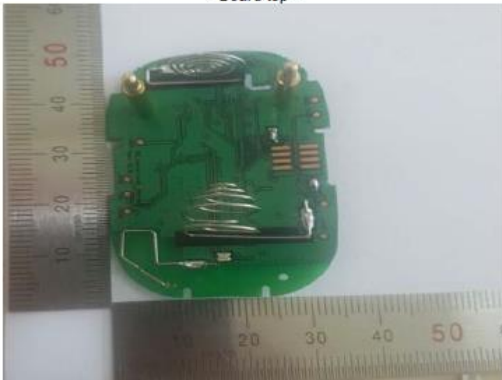
< Board top >
