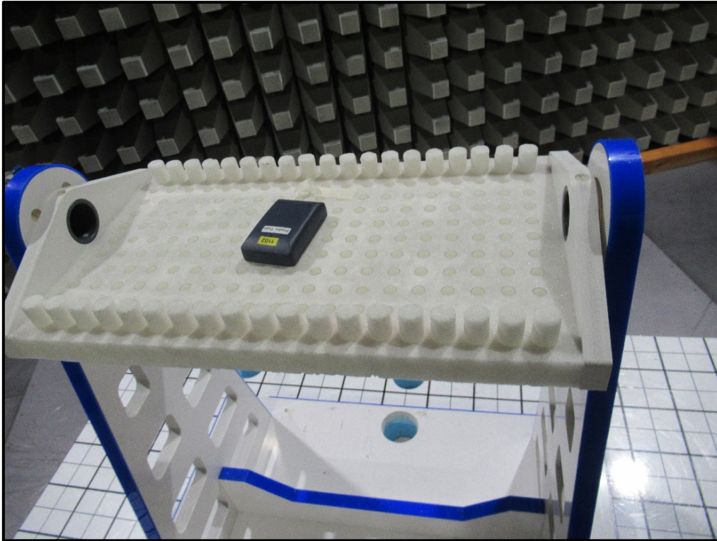
Photo 7: Radiated Test Setup-1 GHz to 10 GHz
