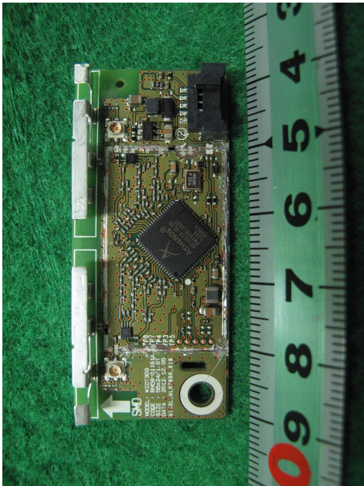
Front Side View of Module without Shielding can
