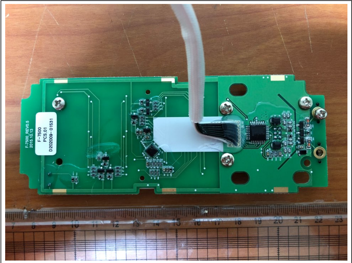
MainBoard-Rear
