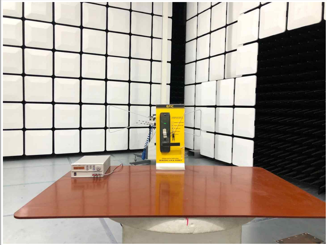
RFID_Radiated Electric Field Emissions Test (Below 1 GHz)
