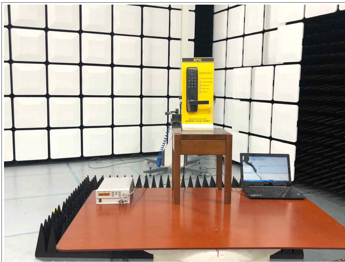
BT_Radiated Electric Field Emissions Test (Above 1GHz)
