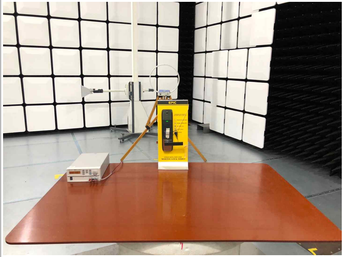
RFID_Radiated Electric Field Emissions Test (Below 30 MHz)
