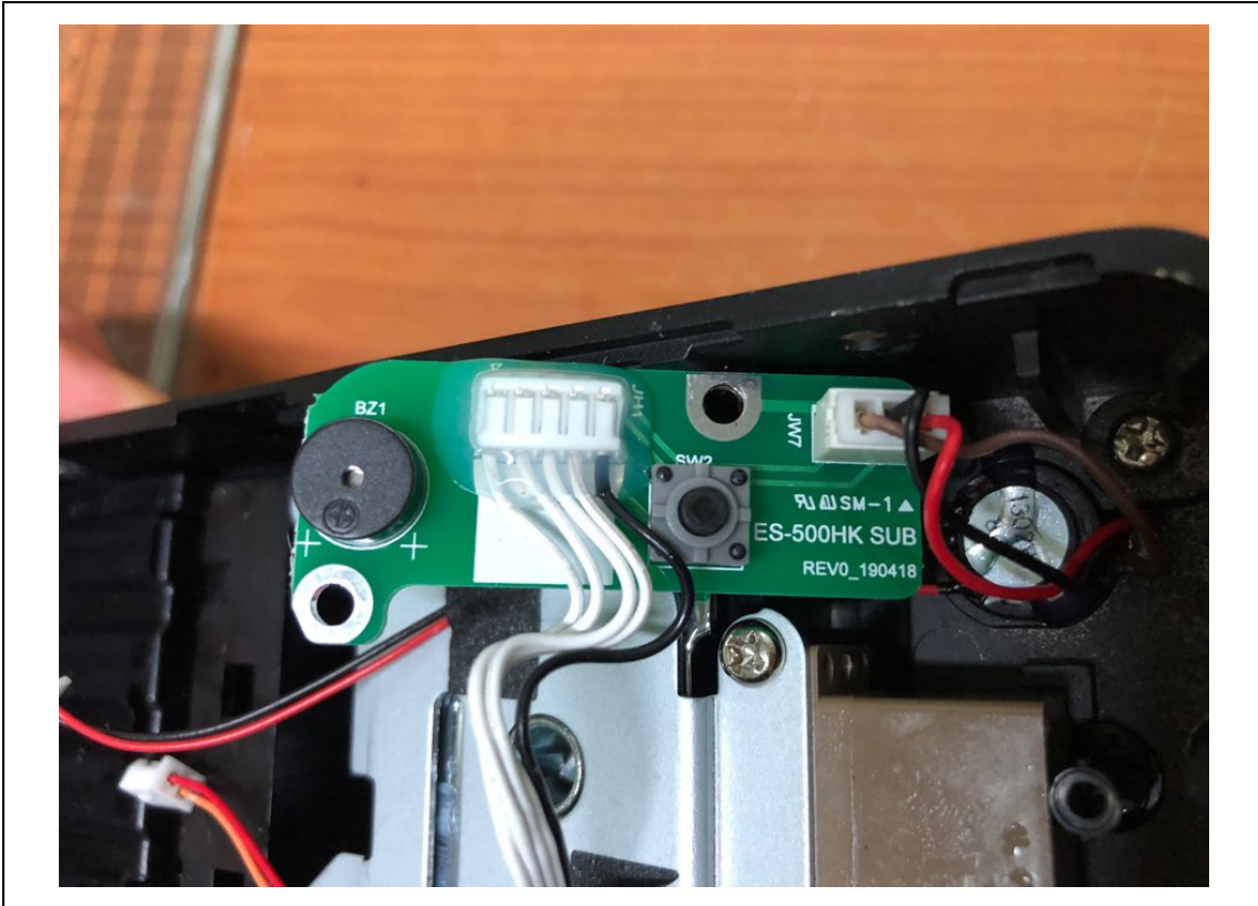
SubBoard-Rear
