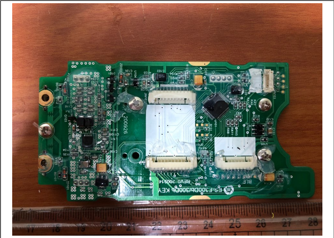
MainBoard-Rear
