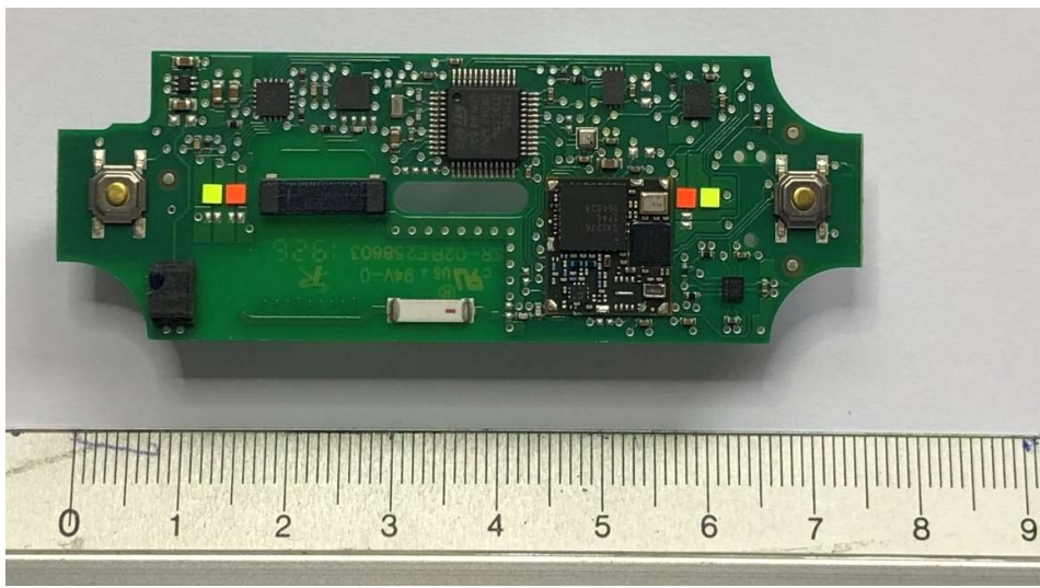
ALOXY Pulse PCB front without cover on Murata module
