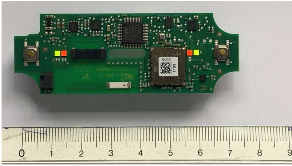
ALOXY Pulse PCB front with cover on Murata module
