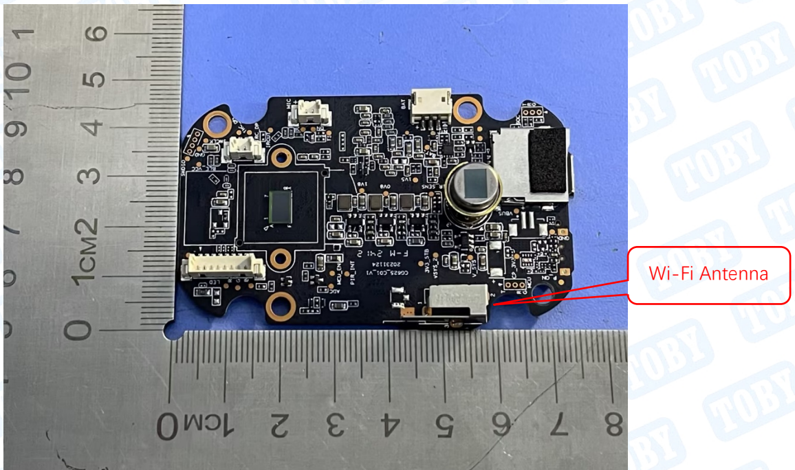
Photo 10 Appearance of PCB
