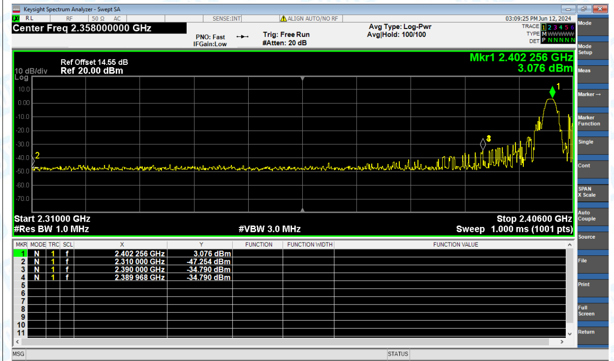
Restrict Band NVNT BLE 1Mbps 2402MHz Ant1 Average
